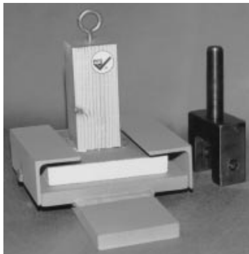
FIG. 1 Tensile Strength Test Specimen Assembly
