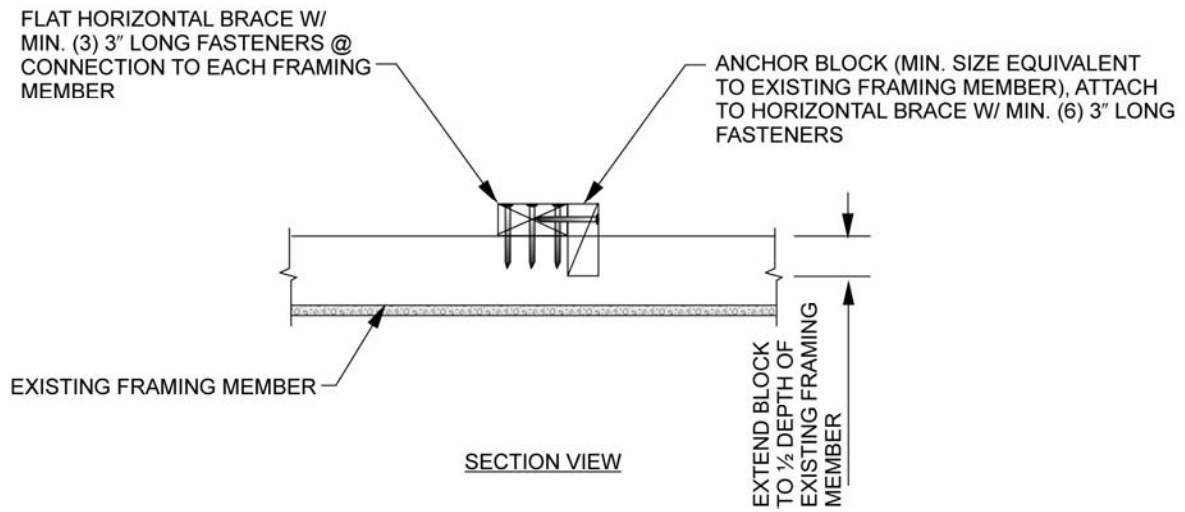
[B] FIGURE C104.2.5 ANCHOR BLOCK INSTALLATION
