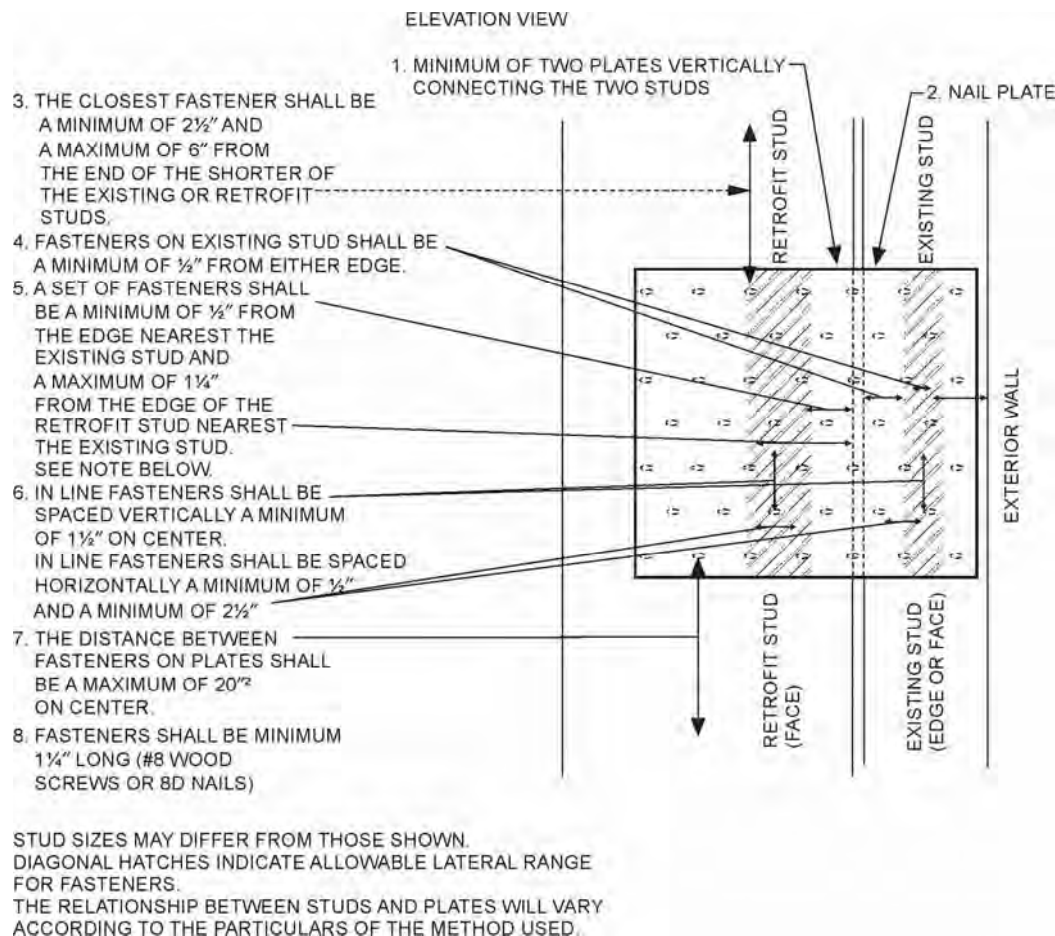
[B] FIGURE C104.3.4 NAIL PLATE FASTENING
