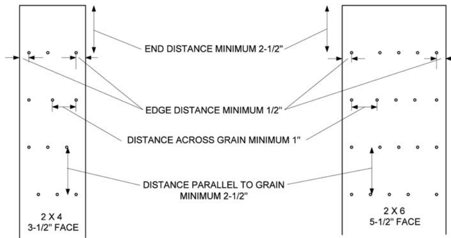
[B] FIGURE C103.6.3 FASTENER SPACINGS FOR LUMBER-TO-LUMBER CONNECTIONS OPERATING IN SHEAR PARALLEL TO GRAIN
