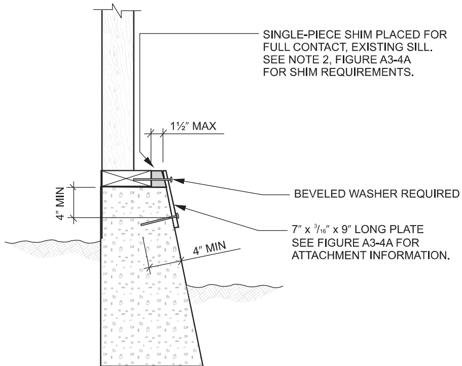
[B] FIGURE A3-4C SILL PLATE ANCHORING TO EXISTING FOUNDATION—ALTERNATE CONNECTION FOR BATTERED FOOTING
