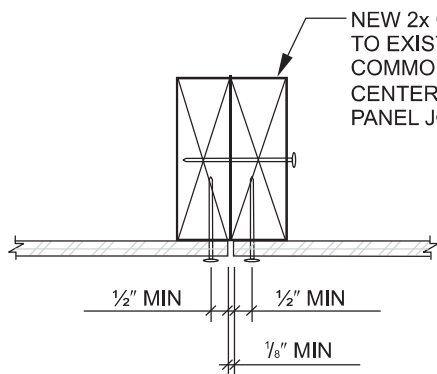
VERTICAL SPLICE AT DOUBLE STUD
