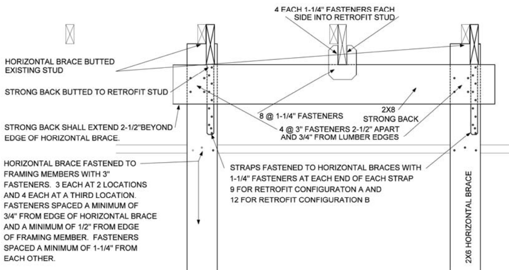
[B] FIGURE C104.2.3 OMITTED HORIZONTAL BRACE
