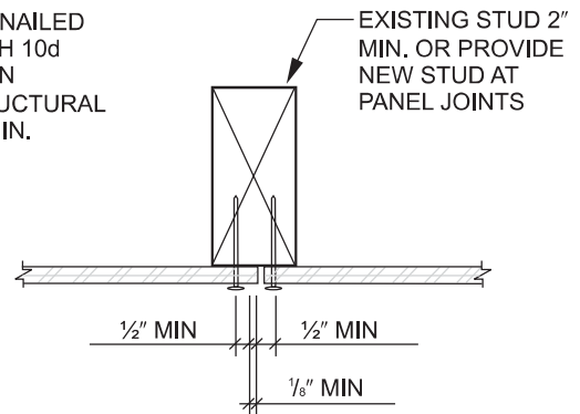
VERTICAL SPLICE AT SINGLE STUD
