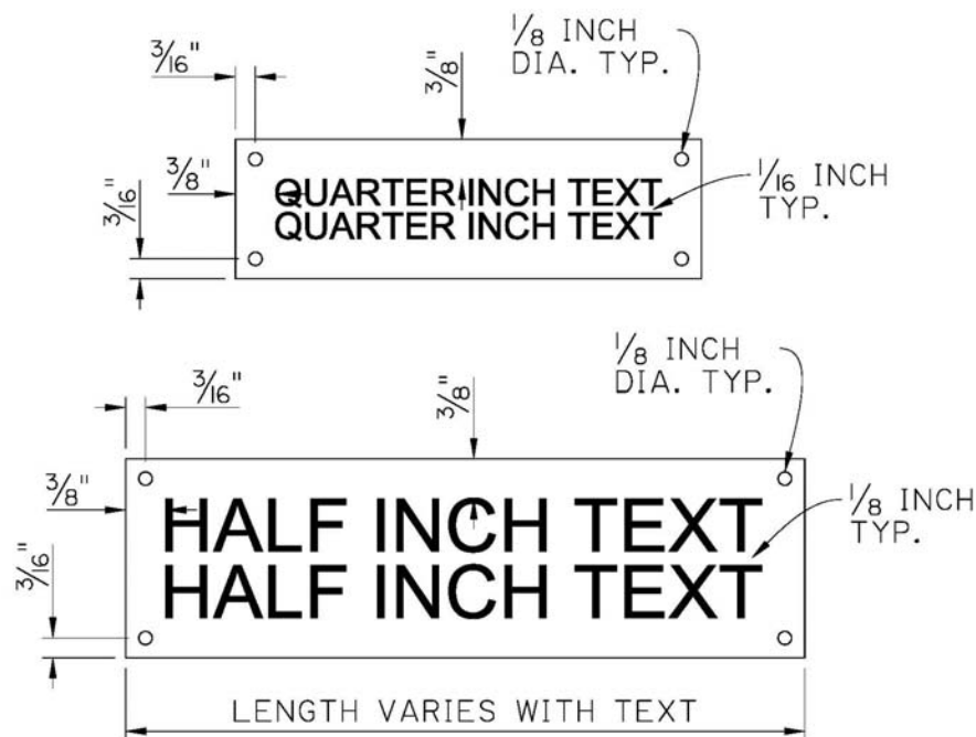
Figure 821.3.070-1 Nameplate Details
