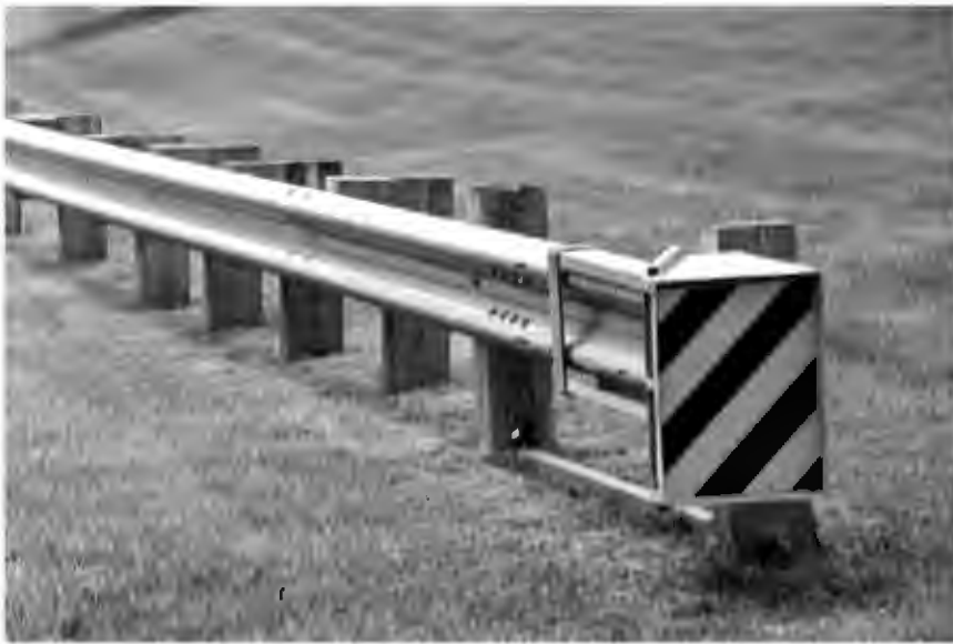
Figure 8-9. Flared Energy-Absorbing Terminal (FLEAT™)
