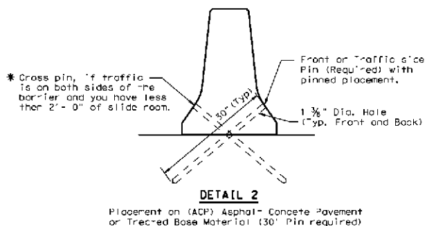
Figure 9-16. TxDOT New Jersey-Shaped Portable Concrete Barrier Pinned-with-Stakes Design
