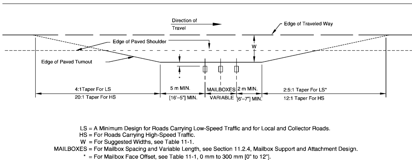
Figure 11-5. Mailbox Turnout
