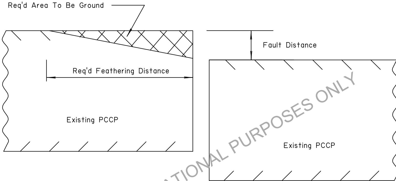
SECTION VIEW
