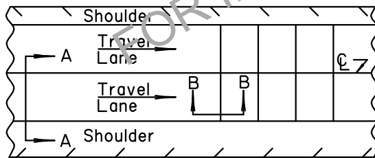
PLAN VIEW
