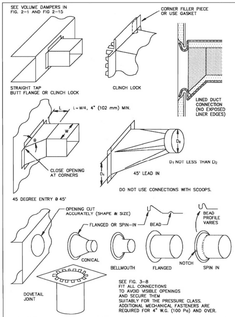
FIG. 2-6 BRANCH CONNECTIONS
