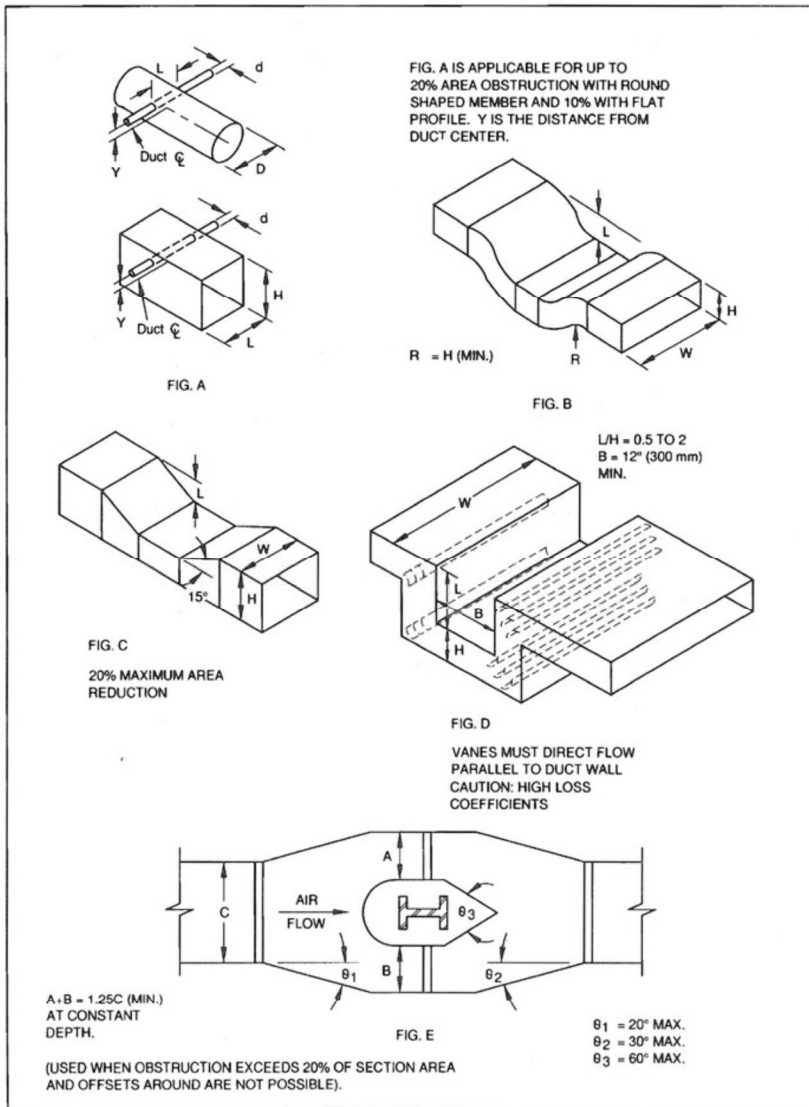
FIG. 2-8 OBSTRUCTIONS
