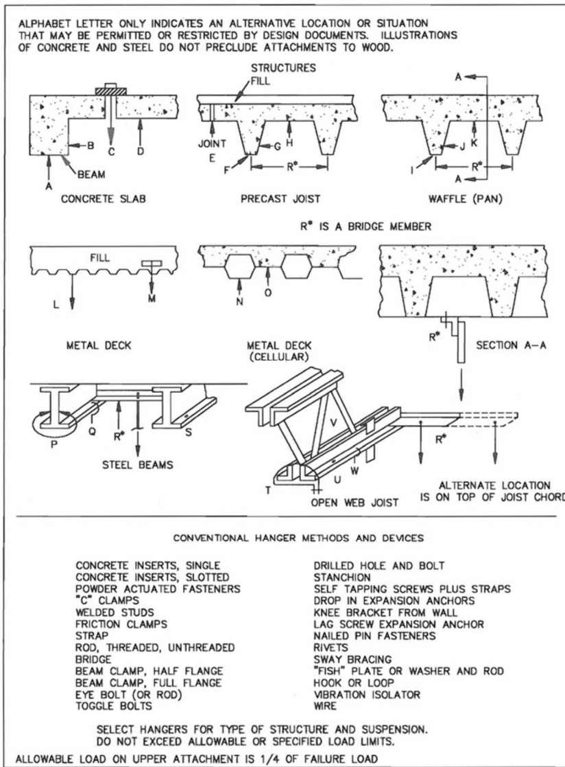
FIG. 4-1 HANGER ATTACHMENTS TO STRUCTURES
