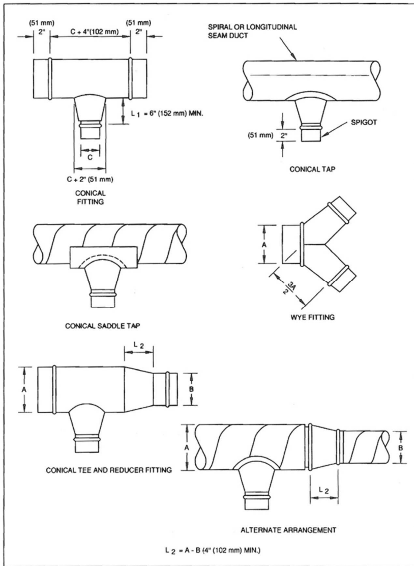
FIG. 3-5 CONICAL TEES
