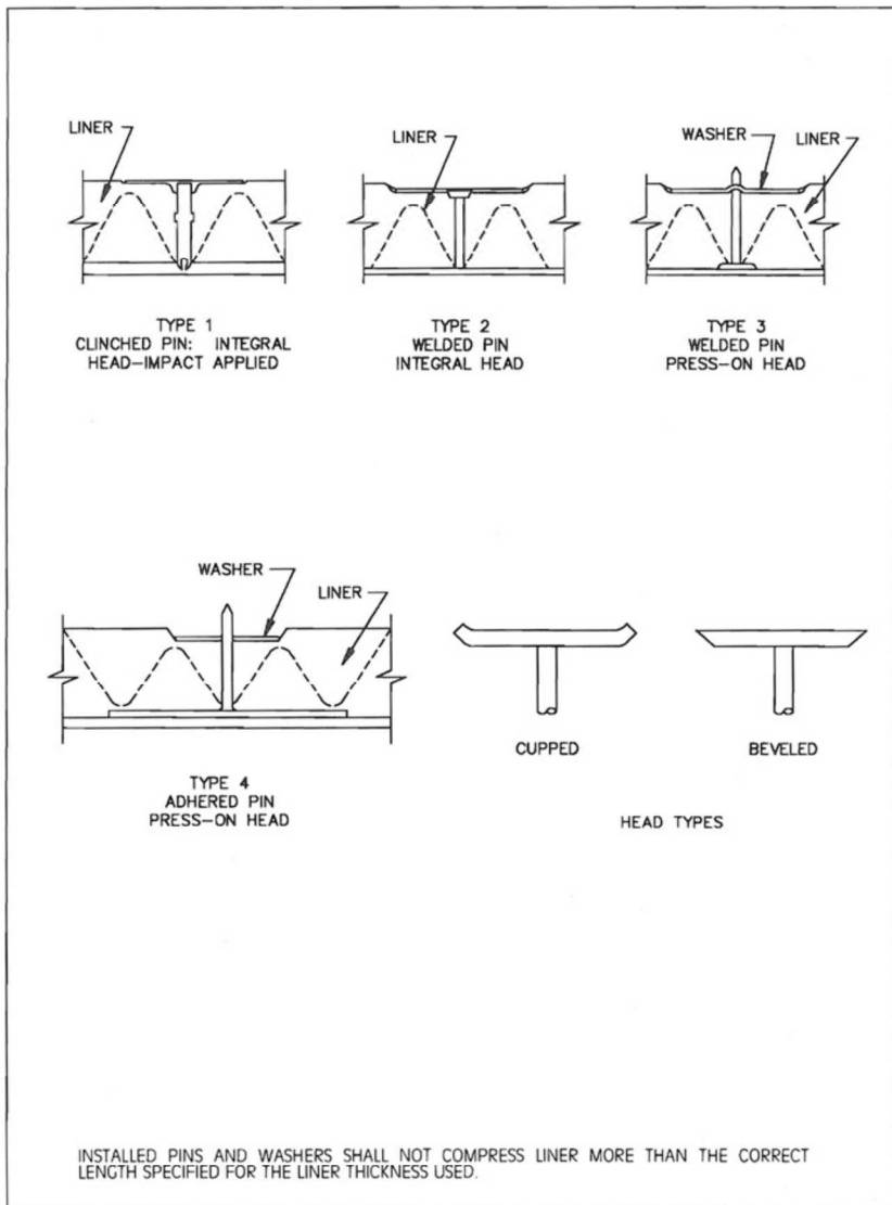
FIG. 2-20 LINER FASTENERS
