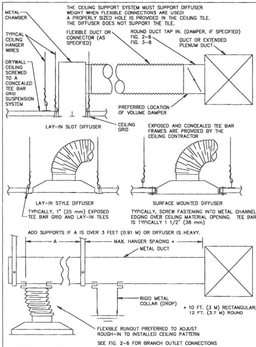
FIG. 2-15 CEILING DIFFUSER BRANCH DUCTS
