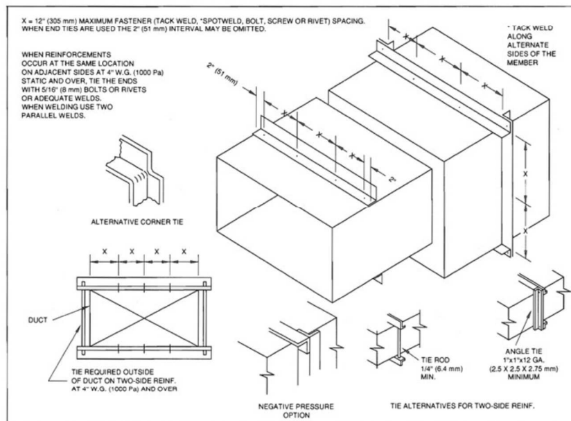
FIG. 1-11 REINFORCEMENT ATTACHMENT
