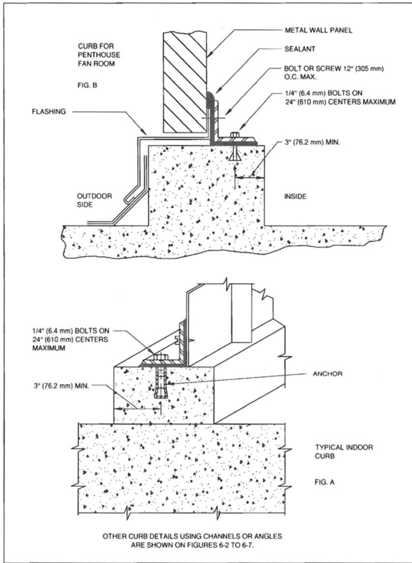
FIG. 6-8 CURB DETAIL
