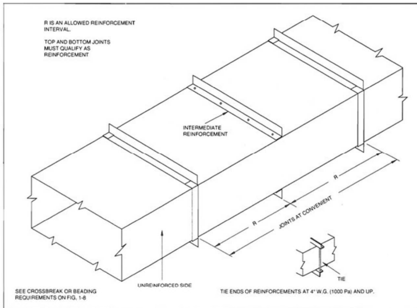
FIG. 1-9 DUCT REINFORCED ON TWO SIDES
