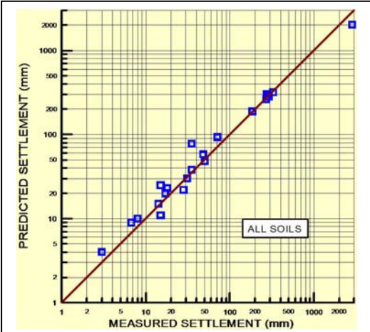
Figure 13: Case studies of settlement prediction using dilatometer tests
