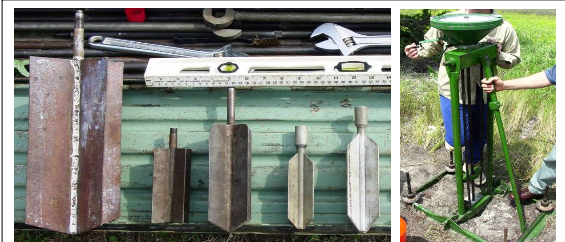
Figure 11: Various size VST shear heads (left) and manual penetration rig with torque head (right)
