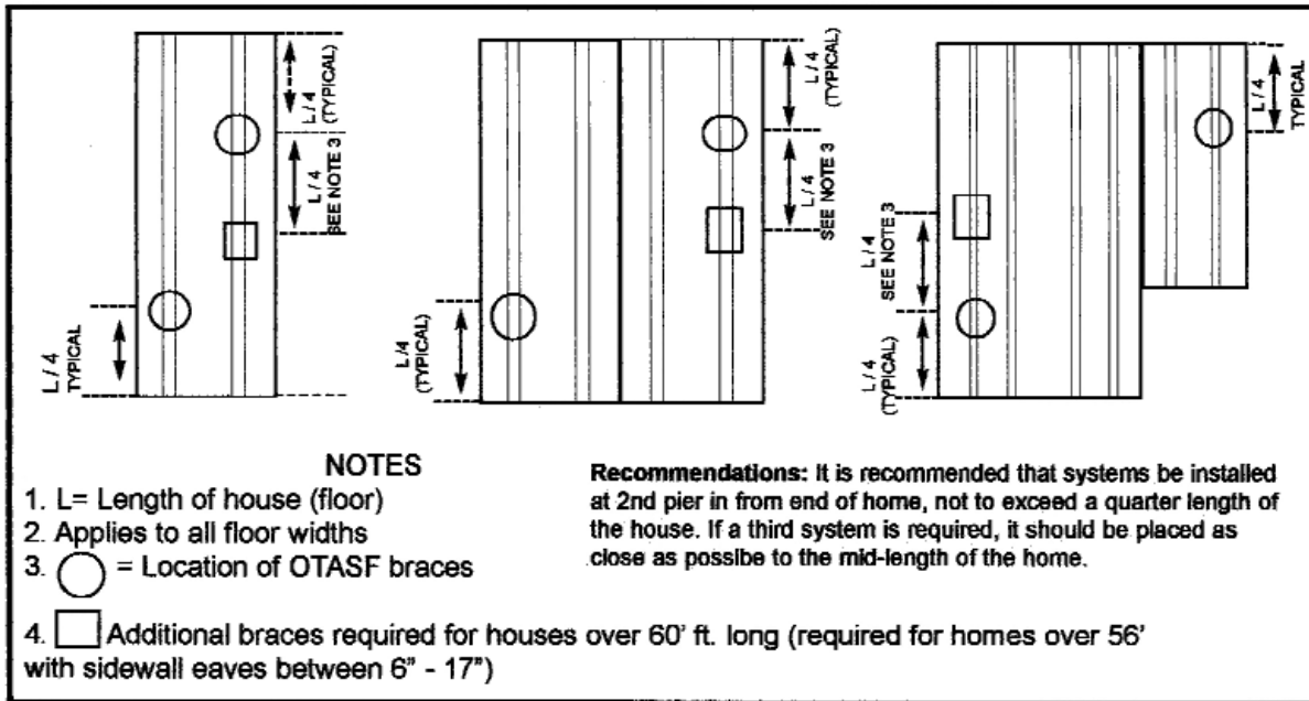
Figure 4.4 Location diagram for Wind Zone I All Steel Foundation System.
