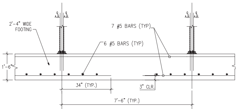
Figure 4.31 Typical continuous footer in central South Carolina.
