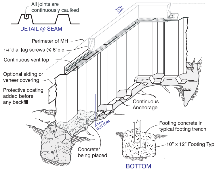
ANCHORPANEL® M.H. FOUNDATION VIEW FROM THE INTERIOR DURING CONCRETE PLACEMENT
