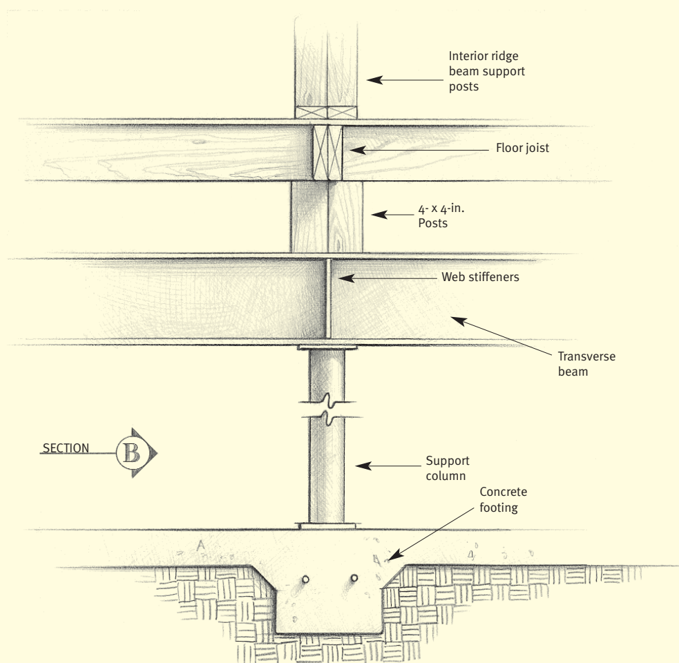
Figure 3.74 Cross section of a home and basement at the centerline showing the column support of the mating wall.
