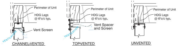
TOP CONNECTION VARIATIONS Cut edges at vents are zinc treated
