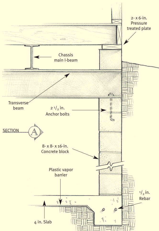
Figure 3.72 Cross section of the Fleetwood basement showing the consideration depth required for the structural components.
