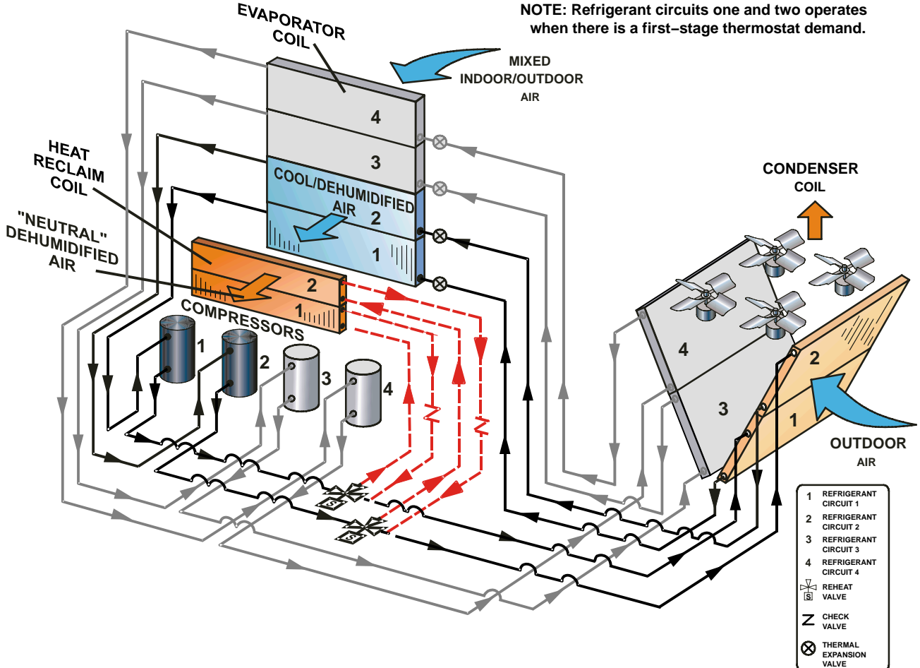
REFRIGERANT SCHEMATIC (210H, 240H and 300S MODELS ONLY)
