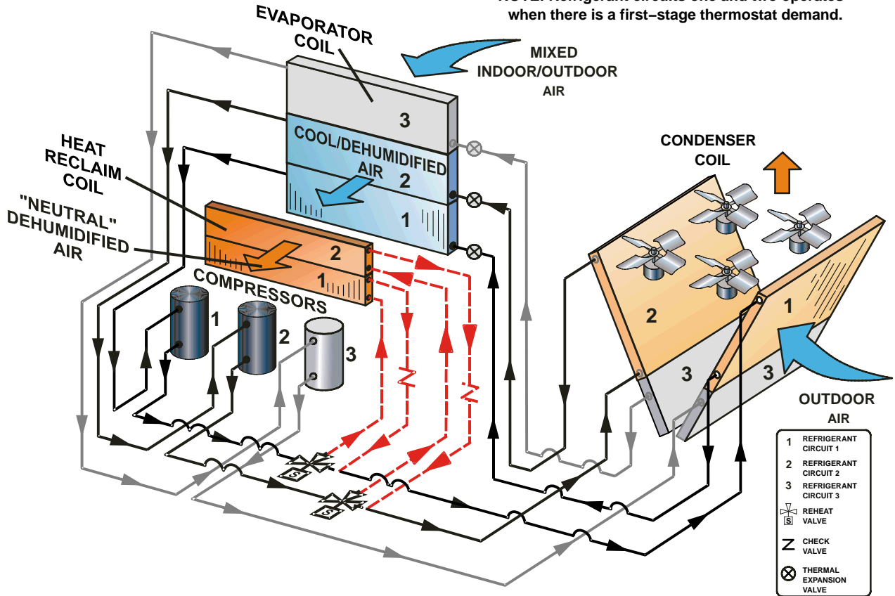
REFRIGERANT SCHEMATIC (210H, 240H and 300S MODELS ONLY)
