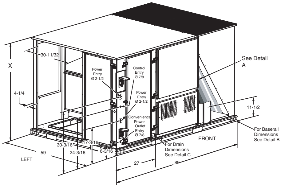
FIGURE 7 - UNIT DIMENSIONS
