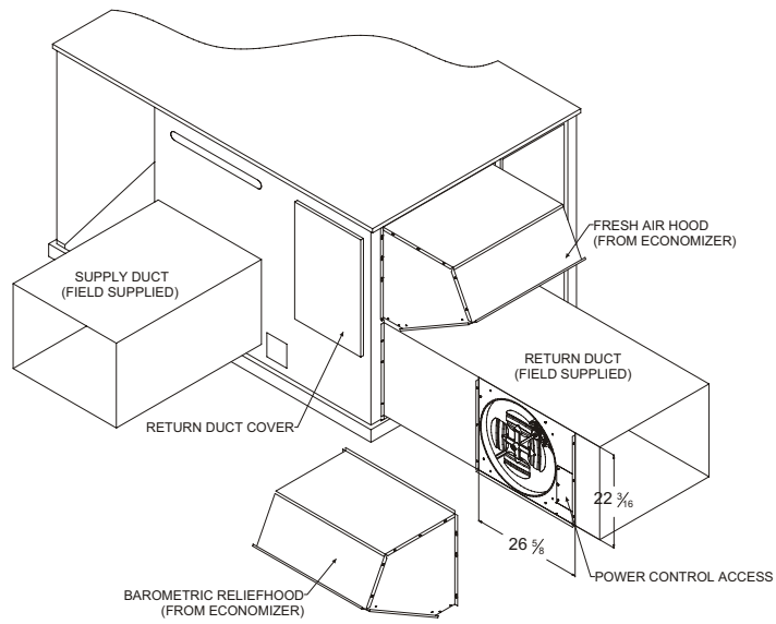
FIGURE 3 - POWER EXHAUST ACCESSORY HORIZONTAL APPLICATION
