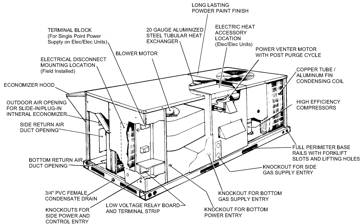
FIGURE 1 - UNIT CUTAWAY
