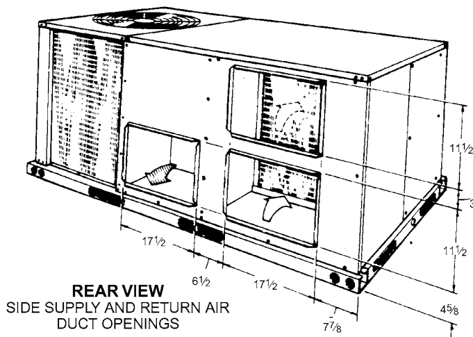
FIGURE 7 - UNIT DIMENSIONS (REAR VIEW)
