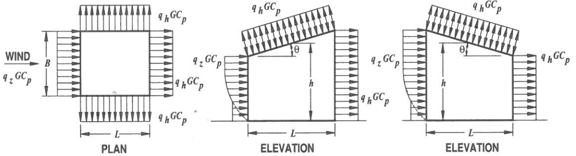
MONSLOPE ROOF (NOTE 4)
