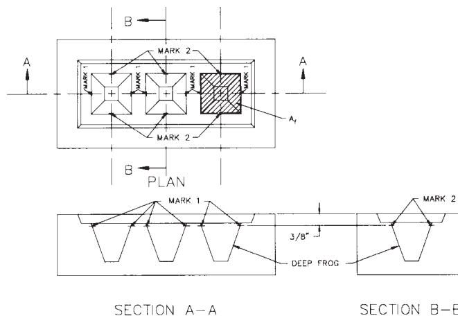
FIG. 3 Deep Frogged Units
