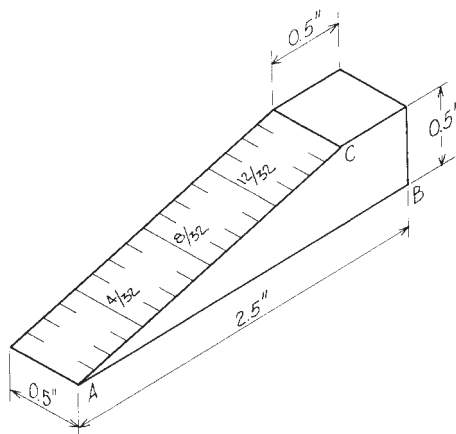
FIG. 1 Measuring Wedge
