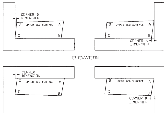
FIG. 4 Out-of-Square Measurements
