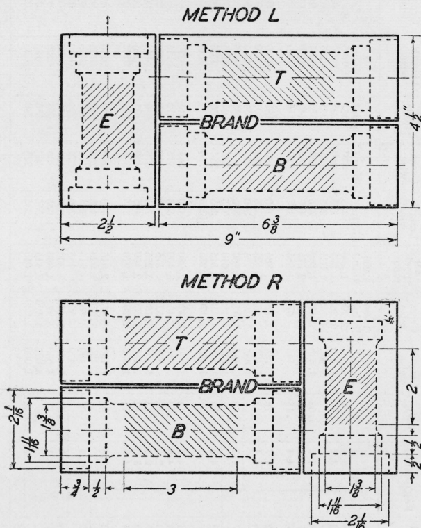
FIGURE 1.—Sections of the brick from which specimens were prepared In each sample of three bricks two were cut by method L and one by method R.
