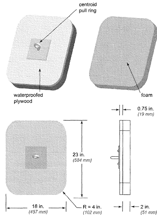
Figure 12: Body Block Element Dimensions
