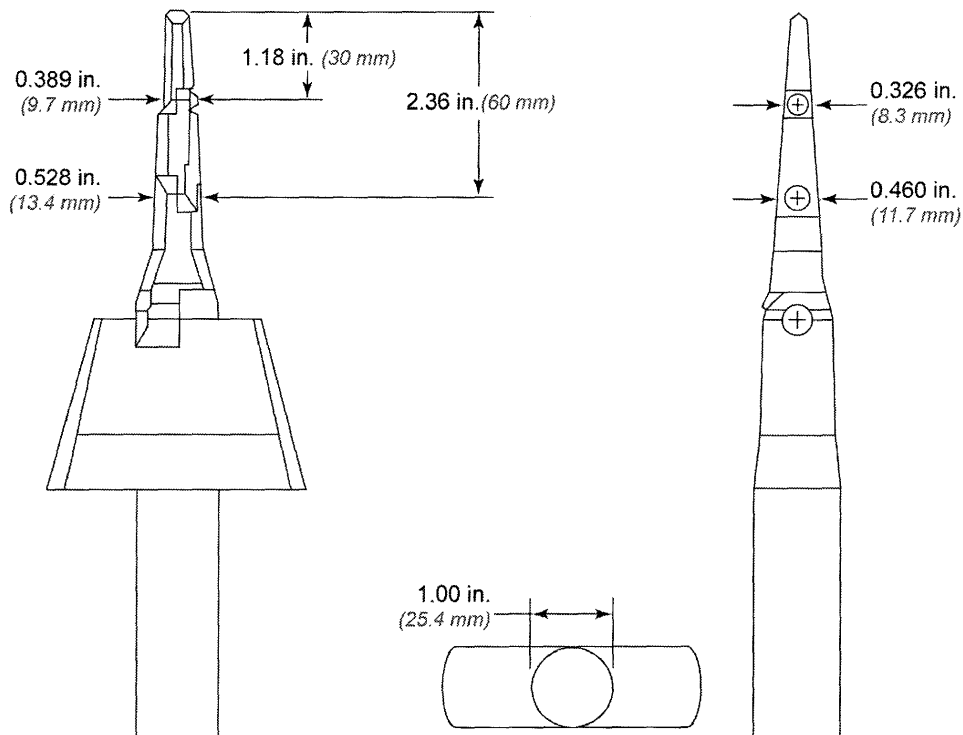
Figure 16: Finger Probe Knuckle Dimensions
