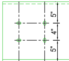
WEB PUNCHING 5/8" x 3/4" SLOTS (STANDARD)
