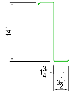
FLANGE PUNCHING 9/16" x 1" SLOTS (OPTIONAL)
