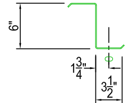
FLANGE PUNCHING 9/16" x 1" SLOTS (OPTIONAL)
