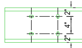
WEB PUNCHING 5/8" x 3/4" SLOTS (STANDARD)
