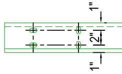
WEB PUNCHING 5/8" x 3/4" SLOTS (STANDARD)
