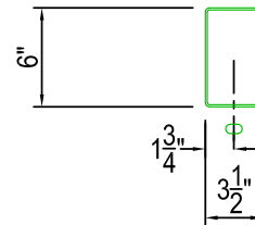
FLANGE PUNCHING 9/16" x 1" SLOTS (OPTIONAL)
