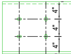
WEB PUNCHING 5/8" x 3/4" SLOTS (STANDARD)
