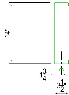
FLANGE PUNCHING 9/16" x 1" SLOTS (OPTIONAL)
