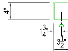
FLANGE PUNCHING 9/16" x 1" SLOTS (OPTIONAL)
