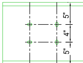
WEB PUNCHING 5/8" x 3/4" SLOTS (STANDARD)
