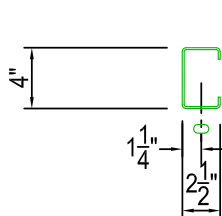
FLANGE PUNCHING 9/16" x 1" SLOTS (OPTIONAL)
