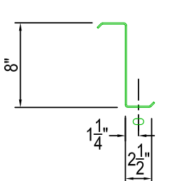
FLANGE PUNCHING 9/16" x 1" SLOTS (OPTIONAL)
