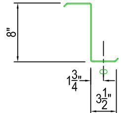
FLANGE PUNCHING 9/16" x 1" SLOTS (OPTIONAL)
