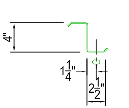
FLANGE PUNCHING 9/16" x 1" SLOTS (OPTIONAL)
