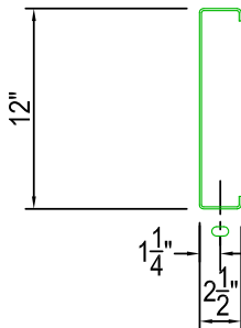
FLANGE PUNCHING 9/16" x 1" SLOTS (OPTIONAL)
