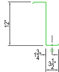
FLANGE PUNCHING 9/16" x 1" SLOTS (OPTIONAL)
