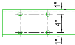
WEB PUNCHING 5/8" x 3/4" SLOTS (STANDARD)
