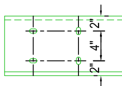
WEB PUNCHING 5/8" x 3/4" SLOTS (STANDARD)
