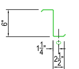
FLANGE PUNCHING 9/16" x 1" SLOTS (OPTIONAL)
