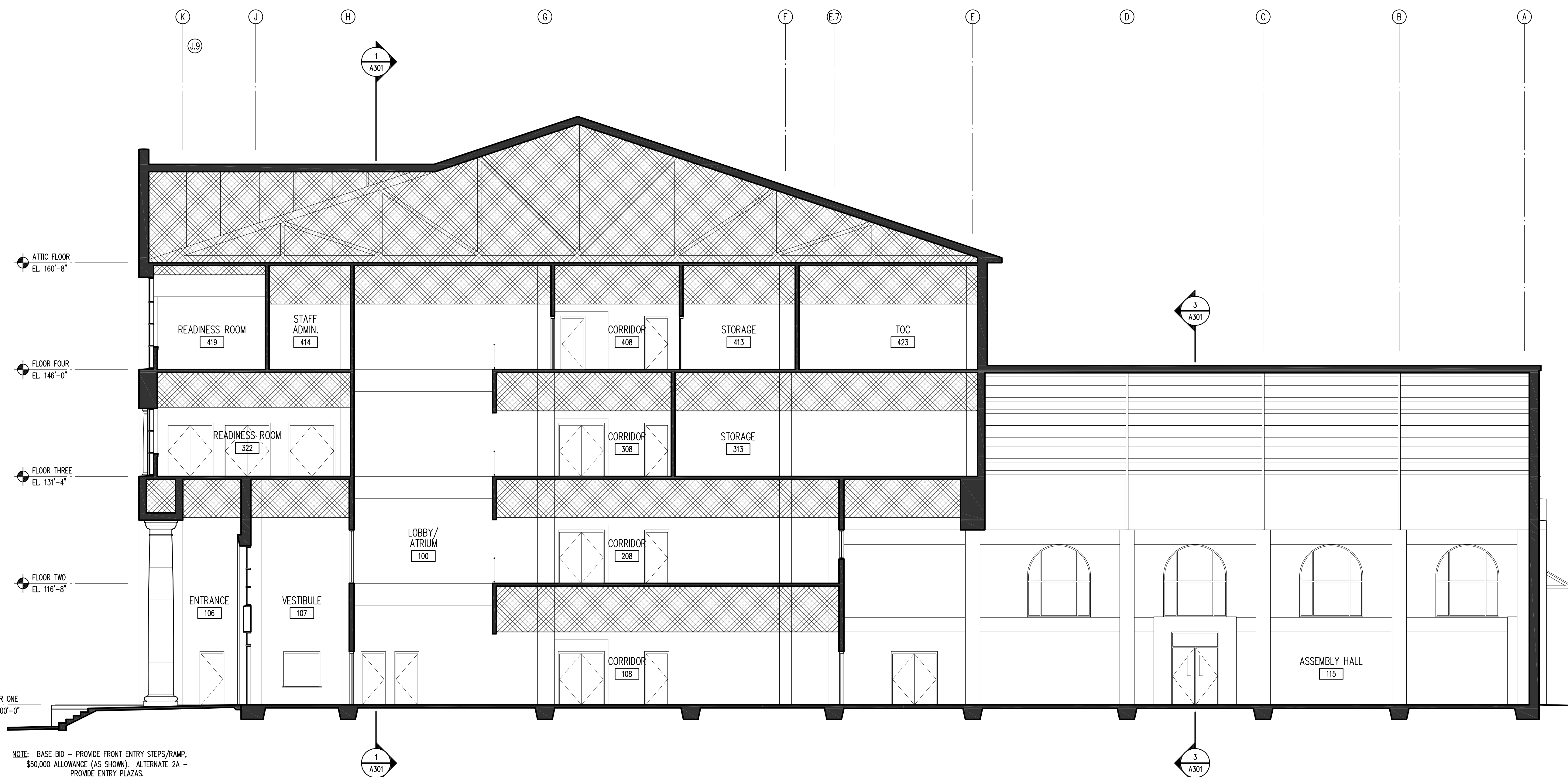
2 TRANSVERSE BLDG. SECTION 1/8" = 1'-0"
