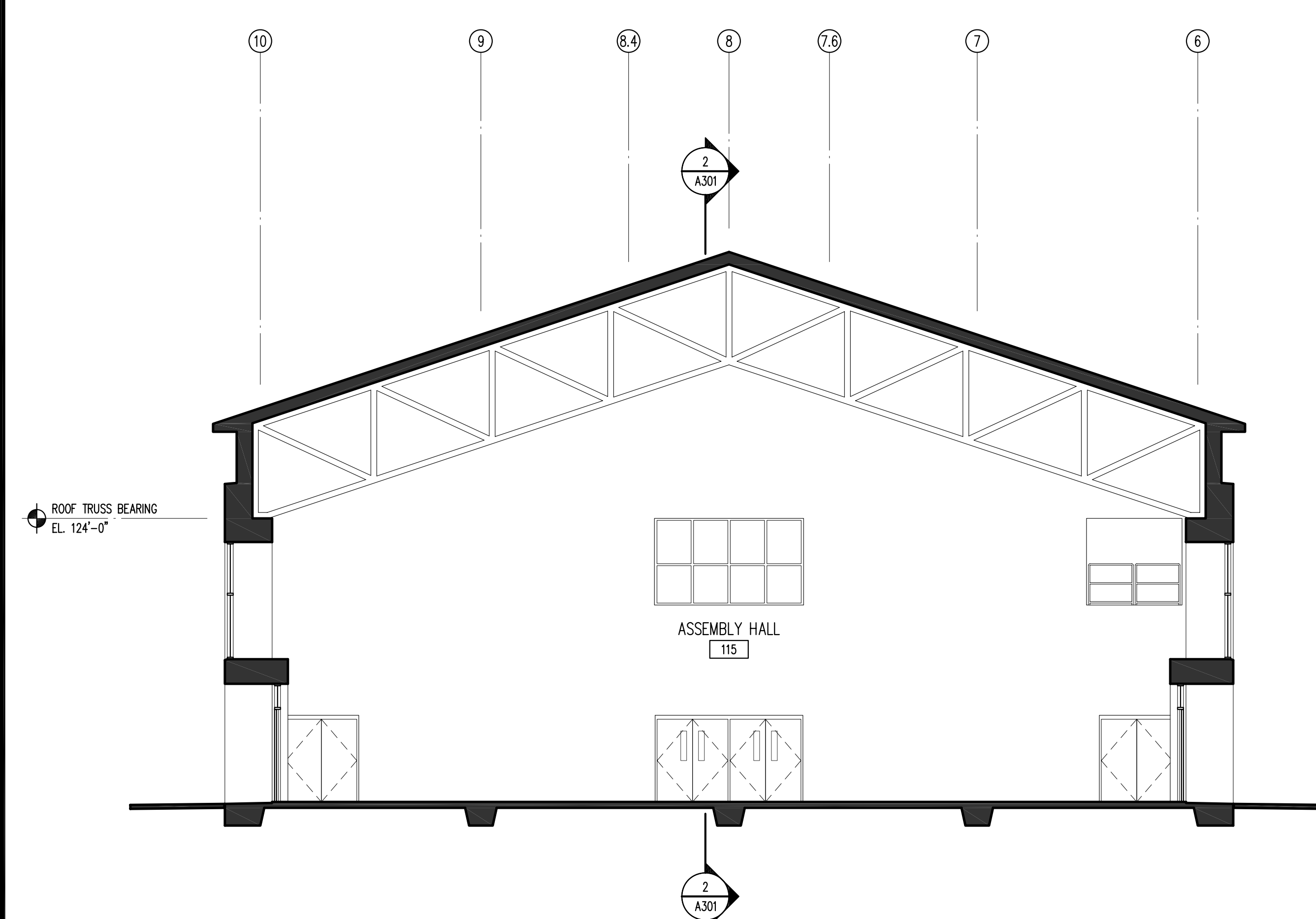
3 ASSEMBLY HALL TRANSV. SECTION 1/8" = 1'-0"
