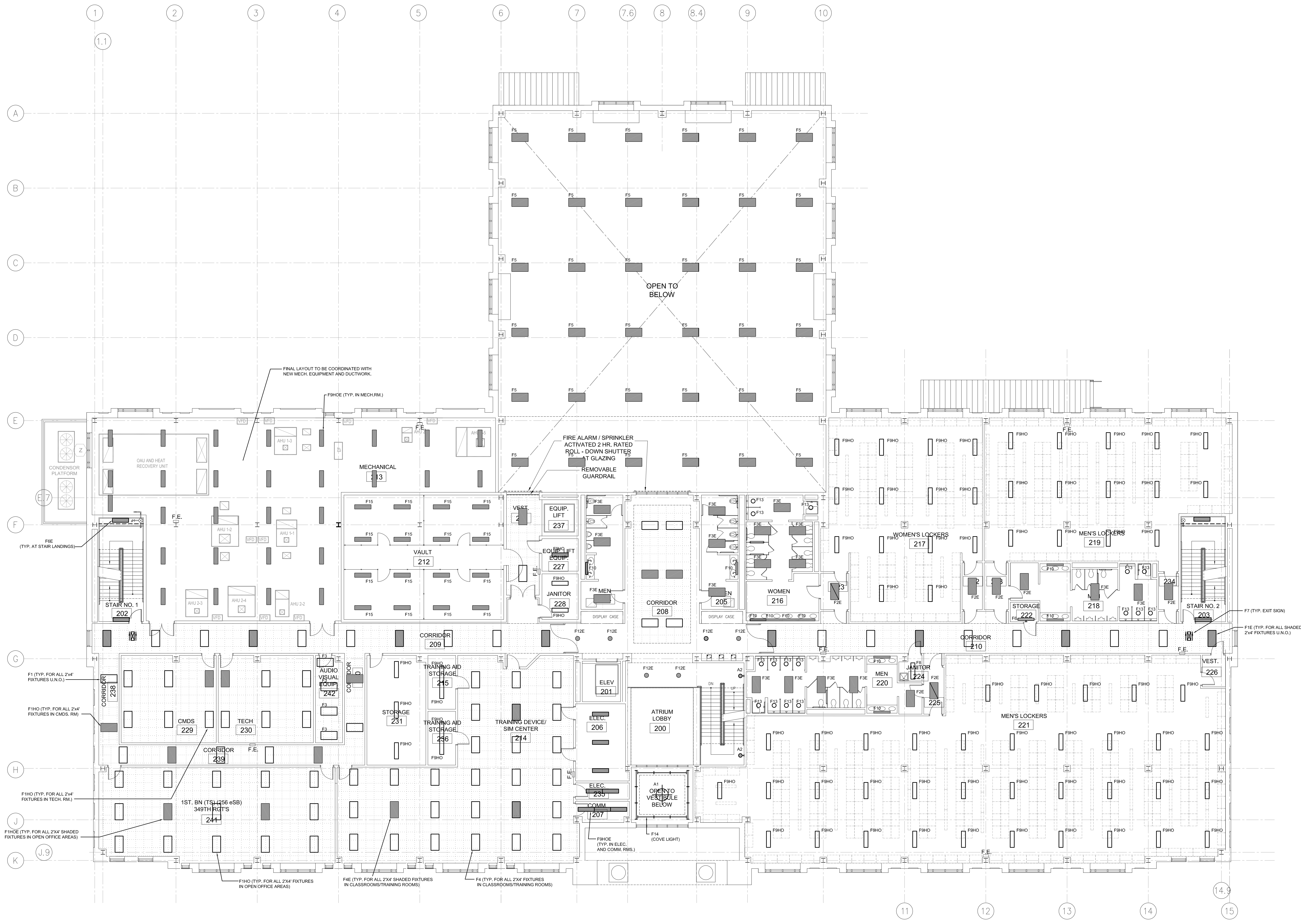
1 LIGHTING PLAN - SECOND FLOOR SCALE 1/8" = 1'-0"
