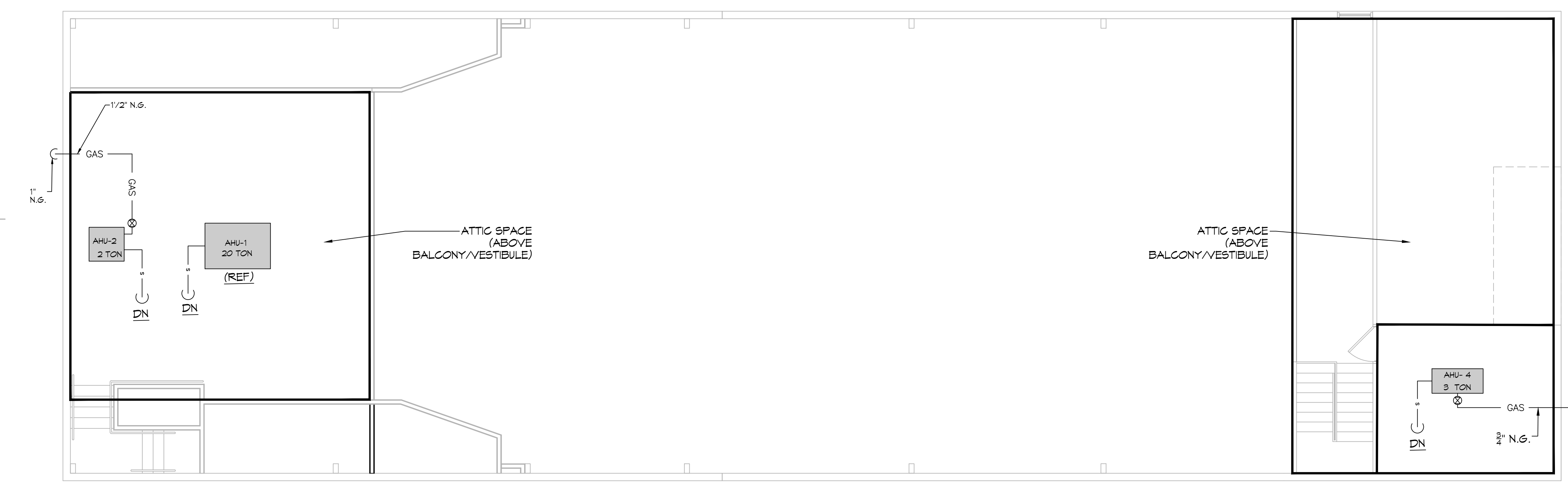
16 SEWER & GAS PLUMBING PLAN SCALE: 3/16"=1'-0" ATTIC
