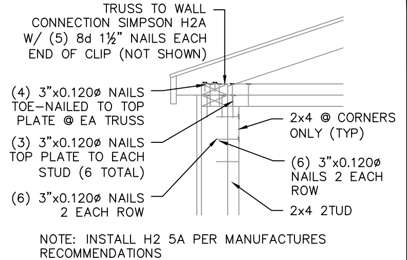
4-CORNER & WALL DETAIL
