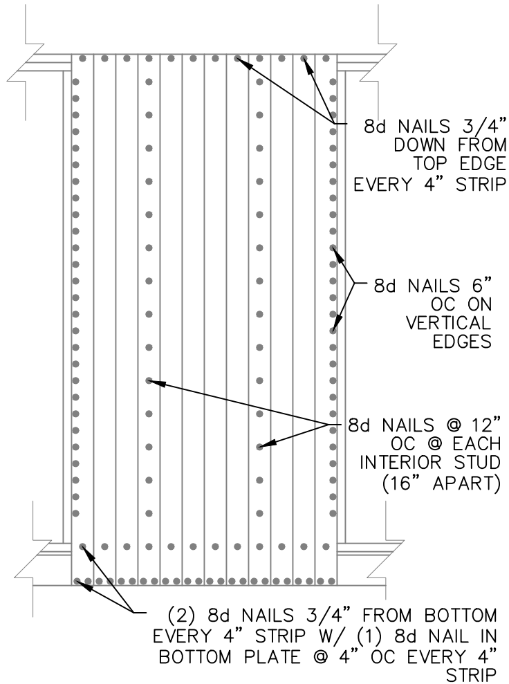
WALL SHEATHING PLAN
