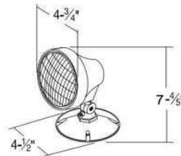
VLL1RGO dimension
