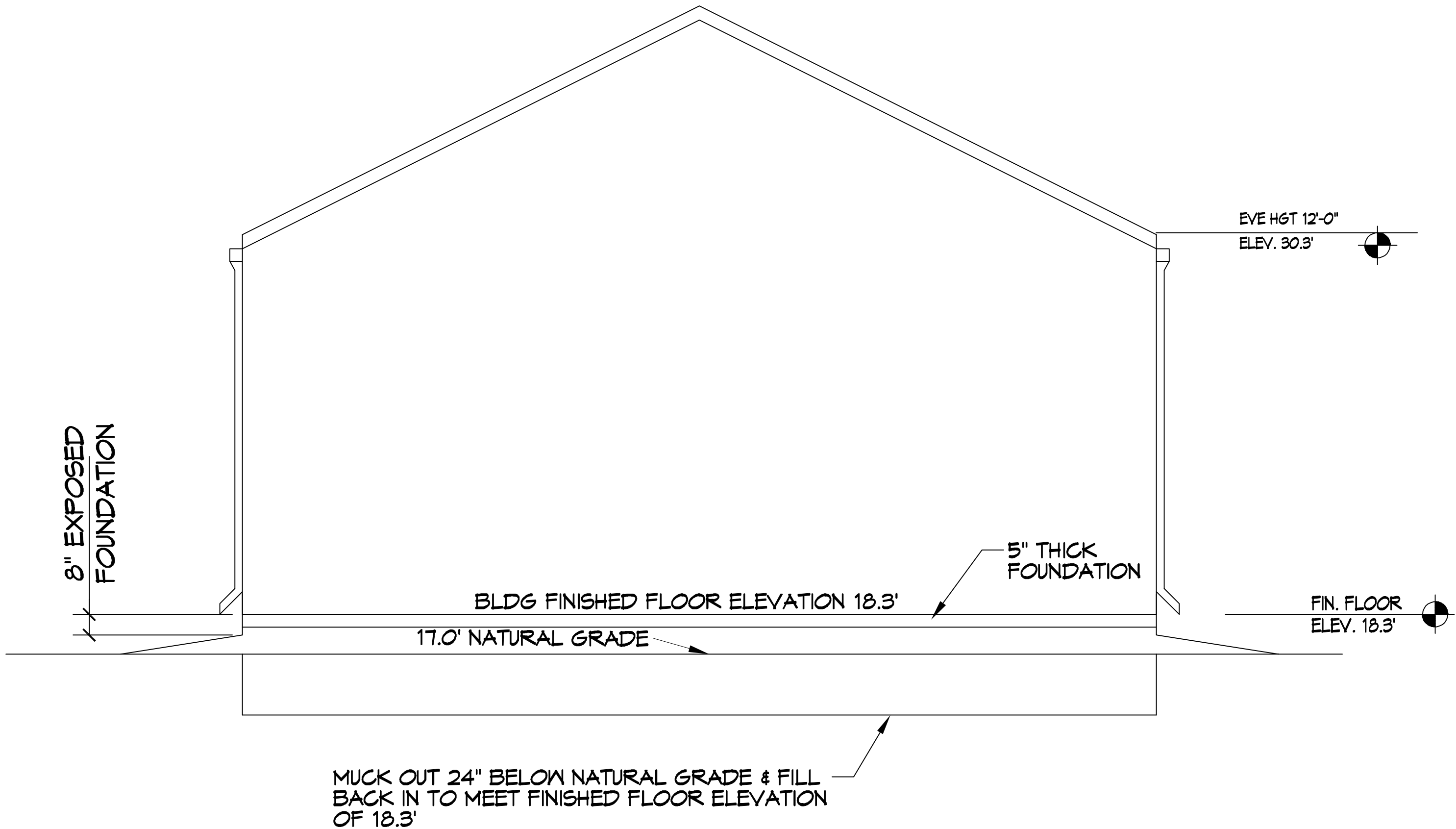
Fill plan drawing
