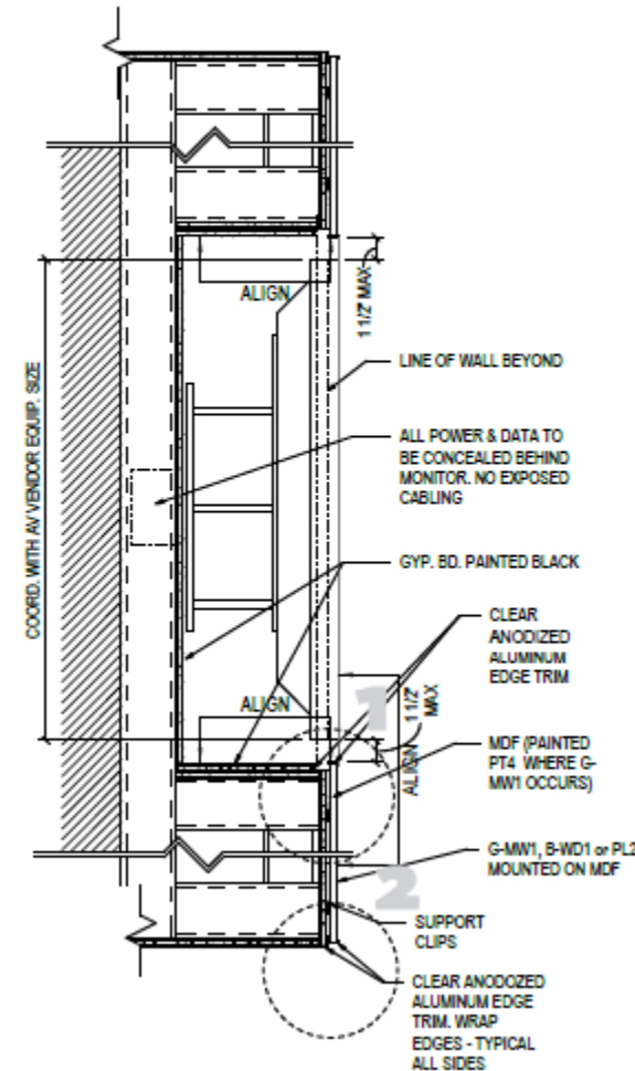
M-3 MILLWORK GMC LIFESTYLE WALL MONITOR PROVIDED BY OTHERS
