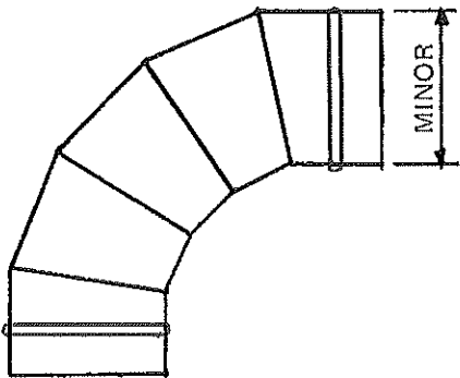
OEL5-90 EASY 5-PIECE 90° ELBOW CENTER LINE RADIUS = 1.5 X MINOR DIMENSION
