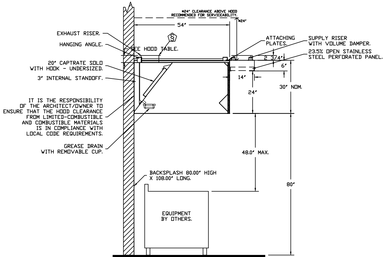
SECTION VIEW - MODEL 5430ND-2-PSP-F HOOD - #1
