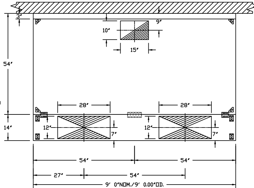
PLAN VIEW - HOOD #1 9' 0.00" LONG 5430ND-2-PSP-F
