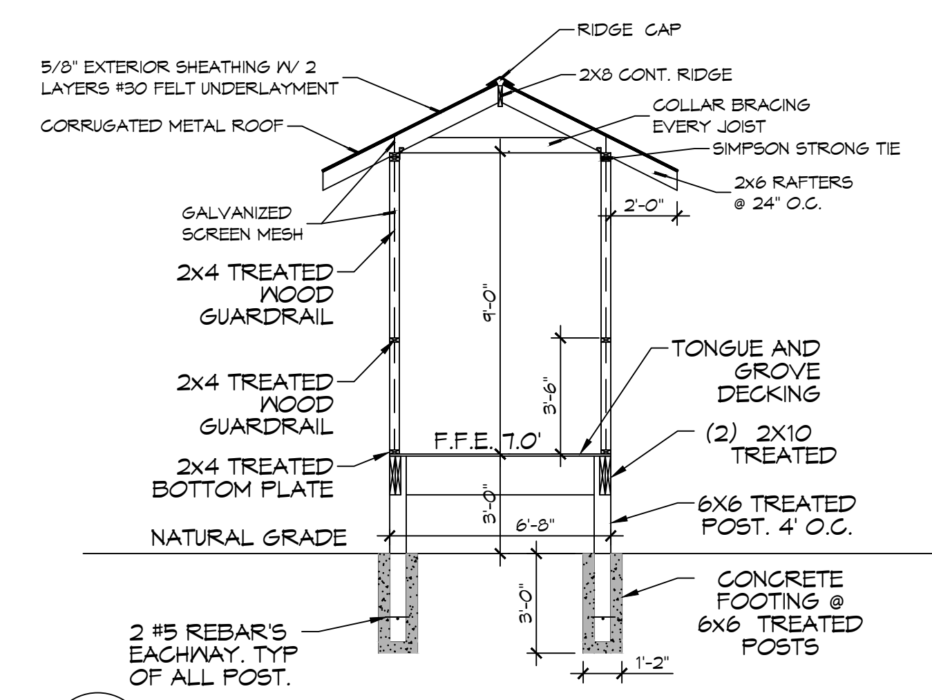
K SECTION SCALE: 3/8" = 1'-0" WALKWAY
