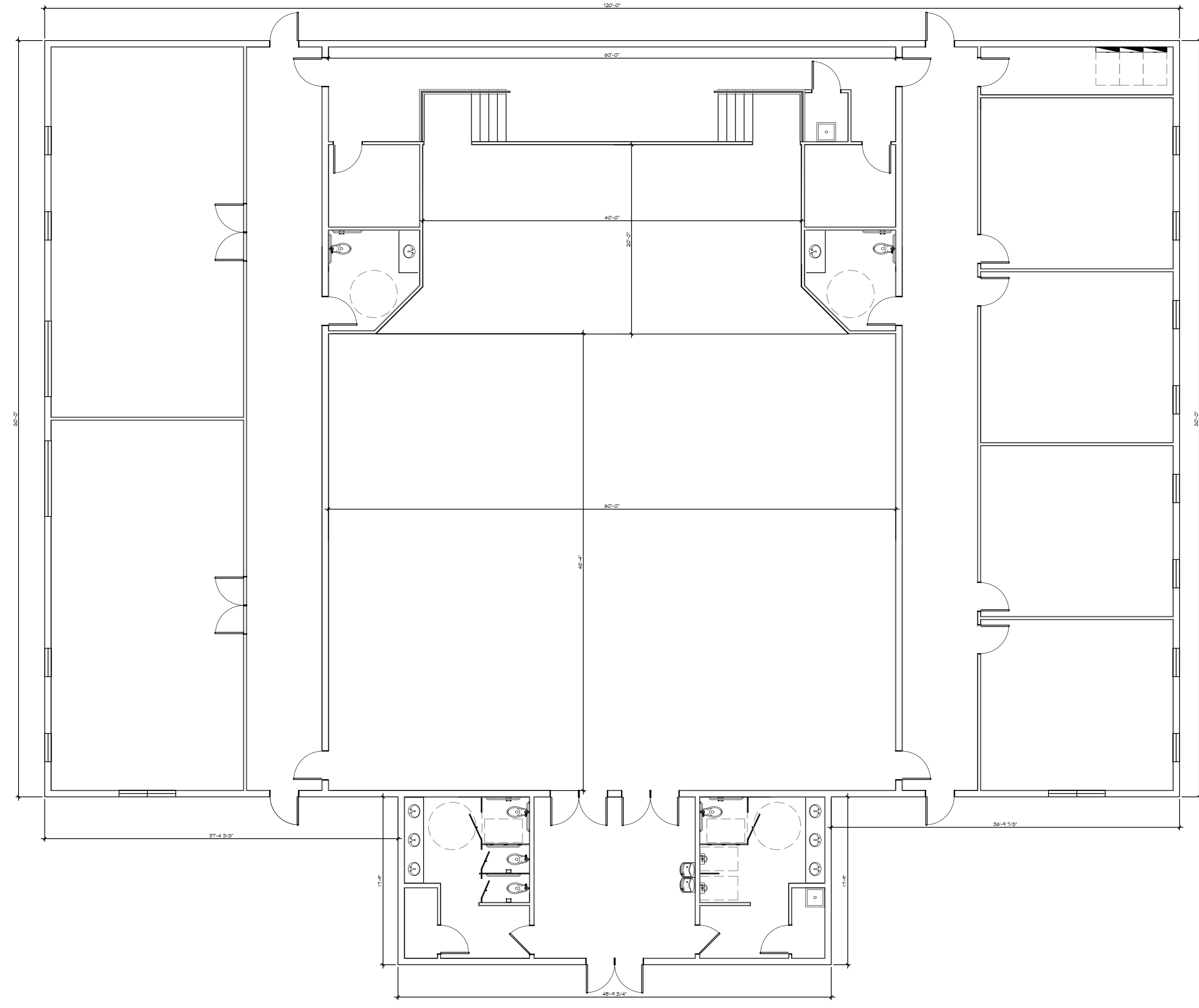
1 FLOOR PLAN SCALE: 1/8"=1'-0"
