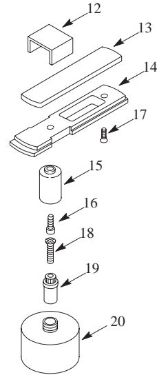
LEVER HANDLE 52700 † LARGE 52701 † SMALL
