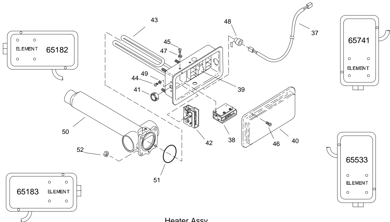
Heater Assy
