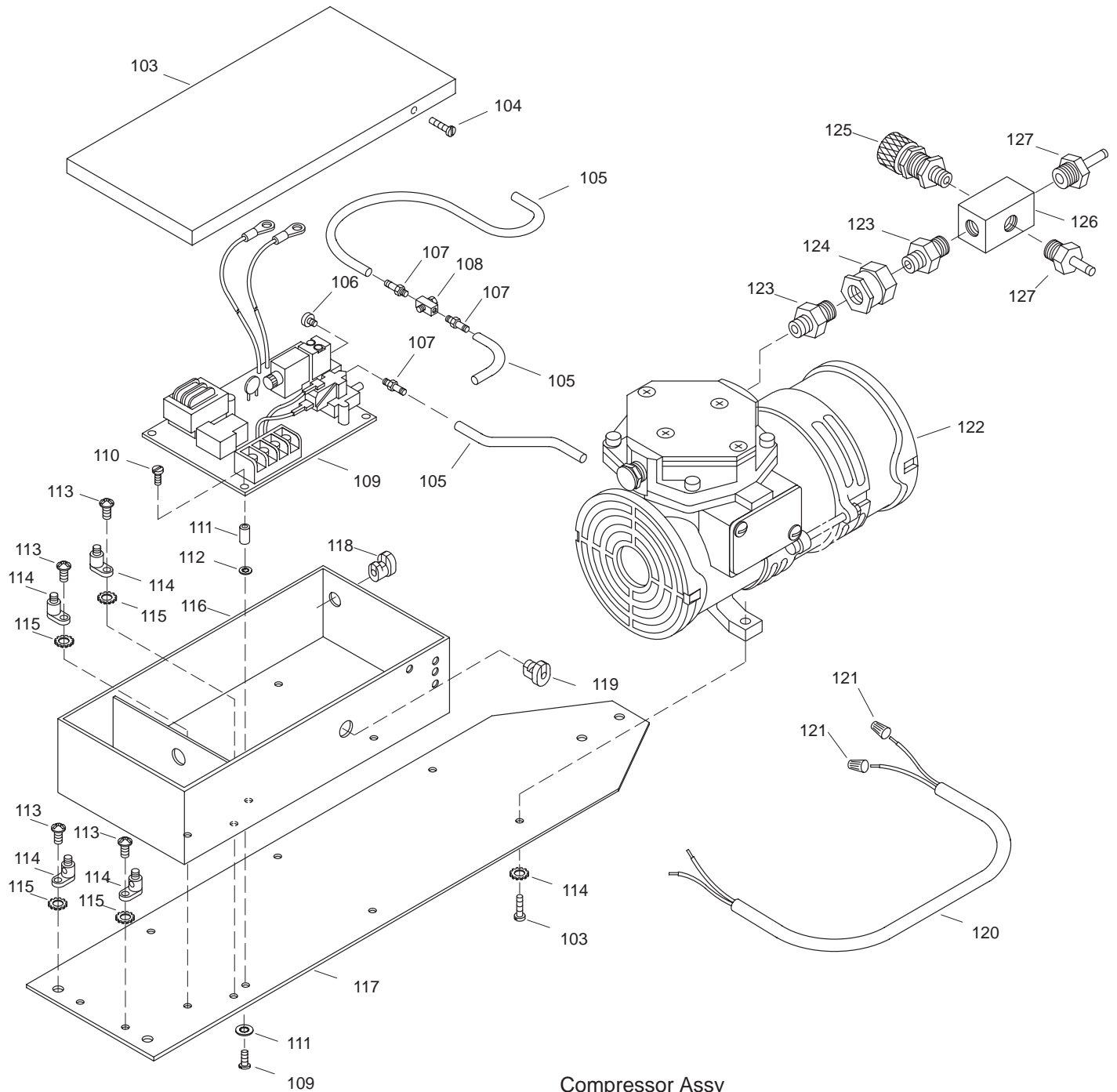
Compressor Assy 97156
