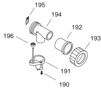
Variable Flow Valve Assy 73592
