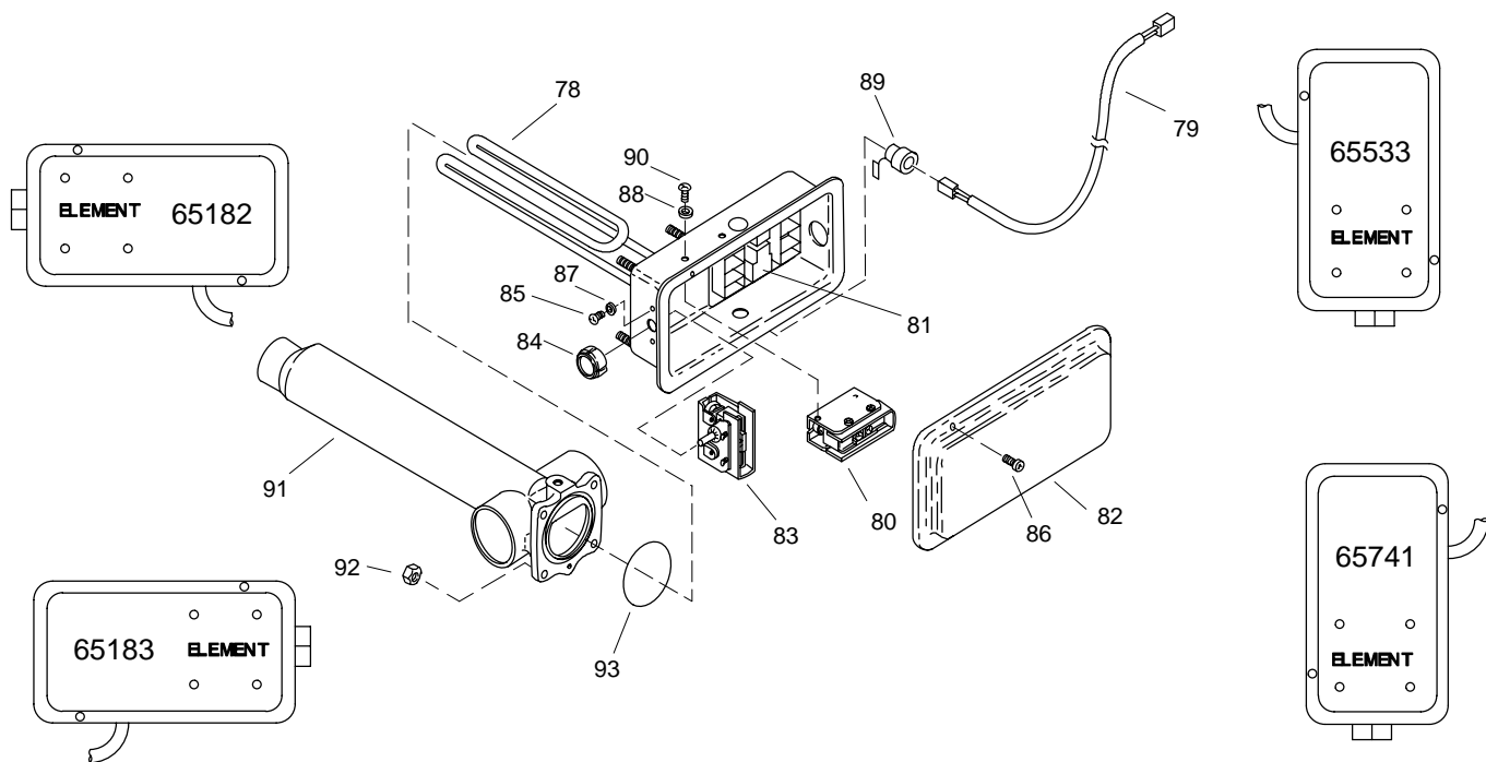
Heater Assy
