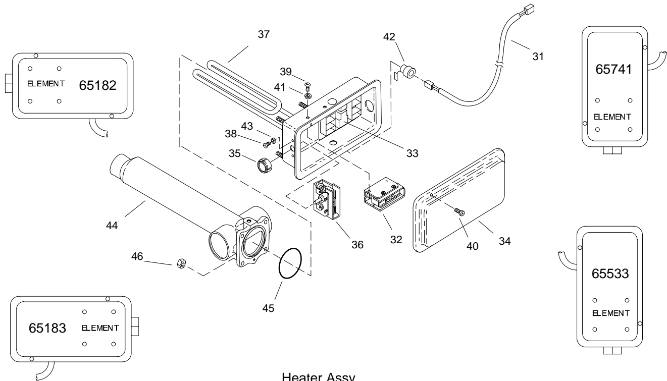
Heater Assy
