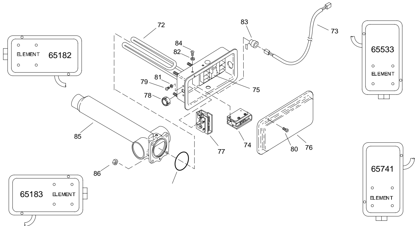
Heater Assy
