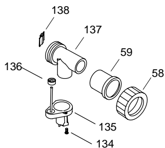
Variable Flow Valve Assy 73592
