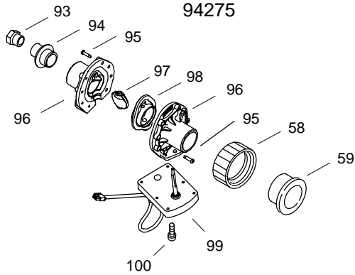
Shut-Off Valve Assy 94275
