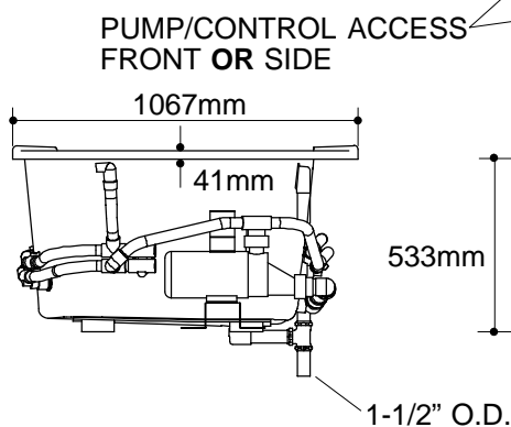
CUT-OUT DETAIL
