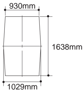
CUT-OUT DETAIL
