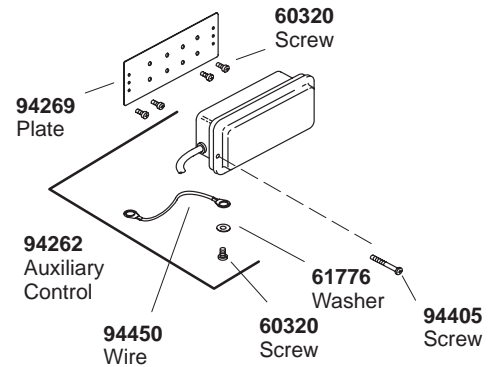
Auxiliary Control Assembly
