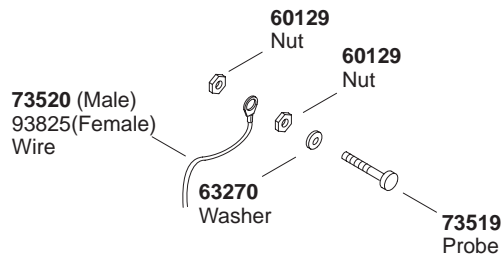
Sensor Probes
