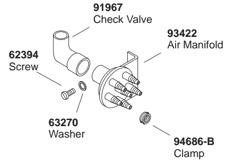
Air Manifold Assembly
