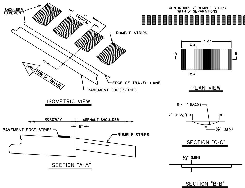
(b) Ground-in Rumble Strips on Asphalt Shoulders
