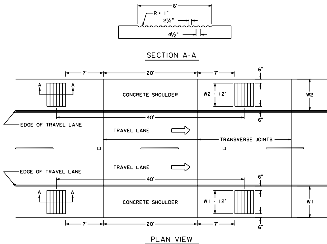
(a) Cast-in Rumble Strips on Concrete Shoulders
