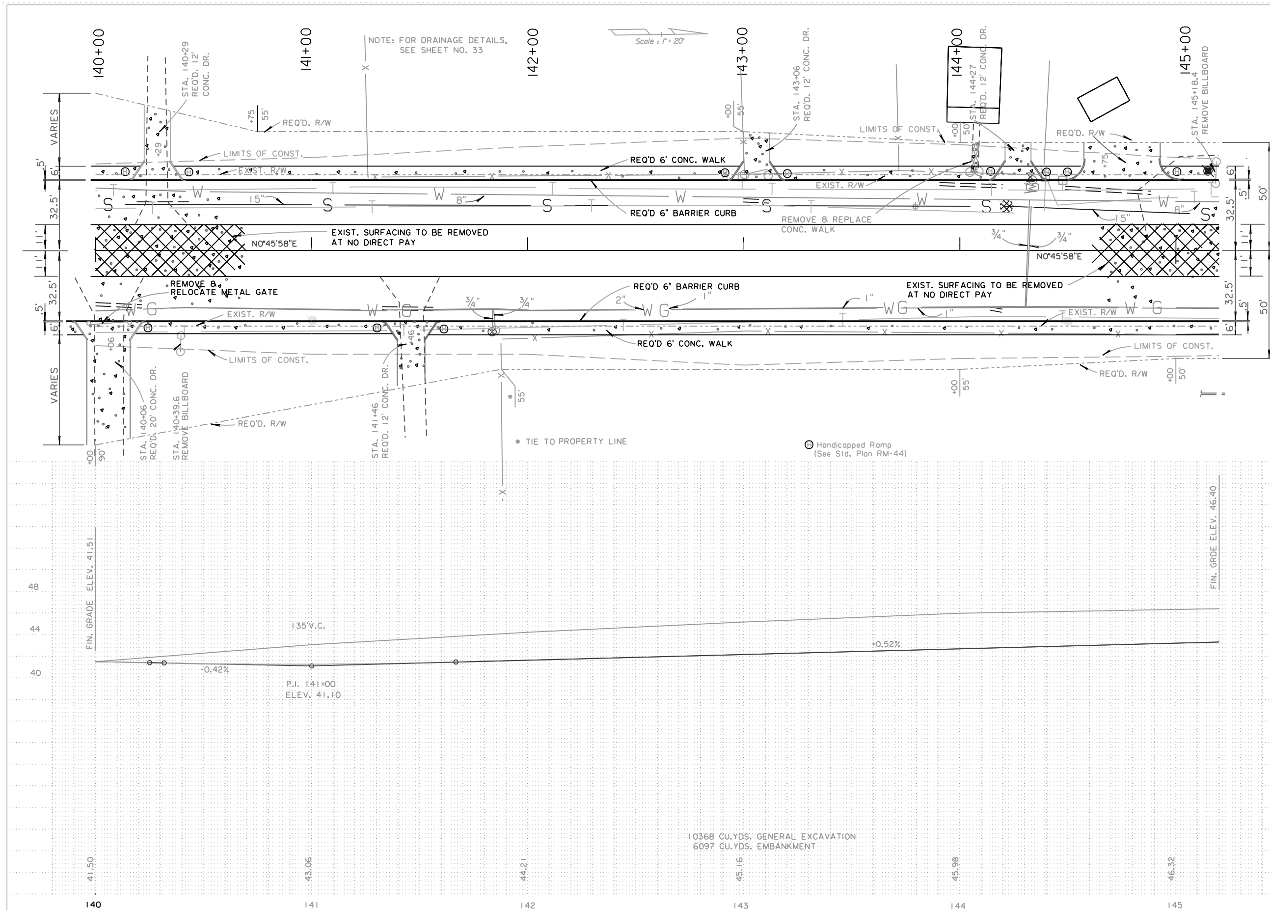
FIGURE 8-36: URBAN PLAN/PROFILE (FINAL)
