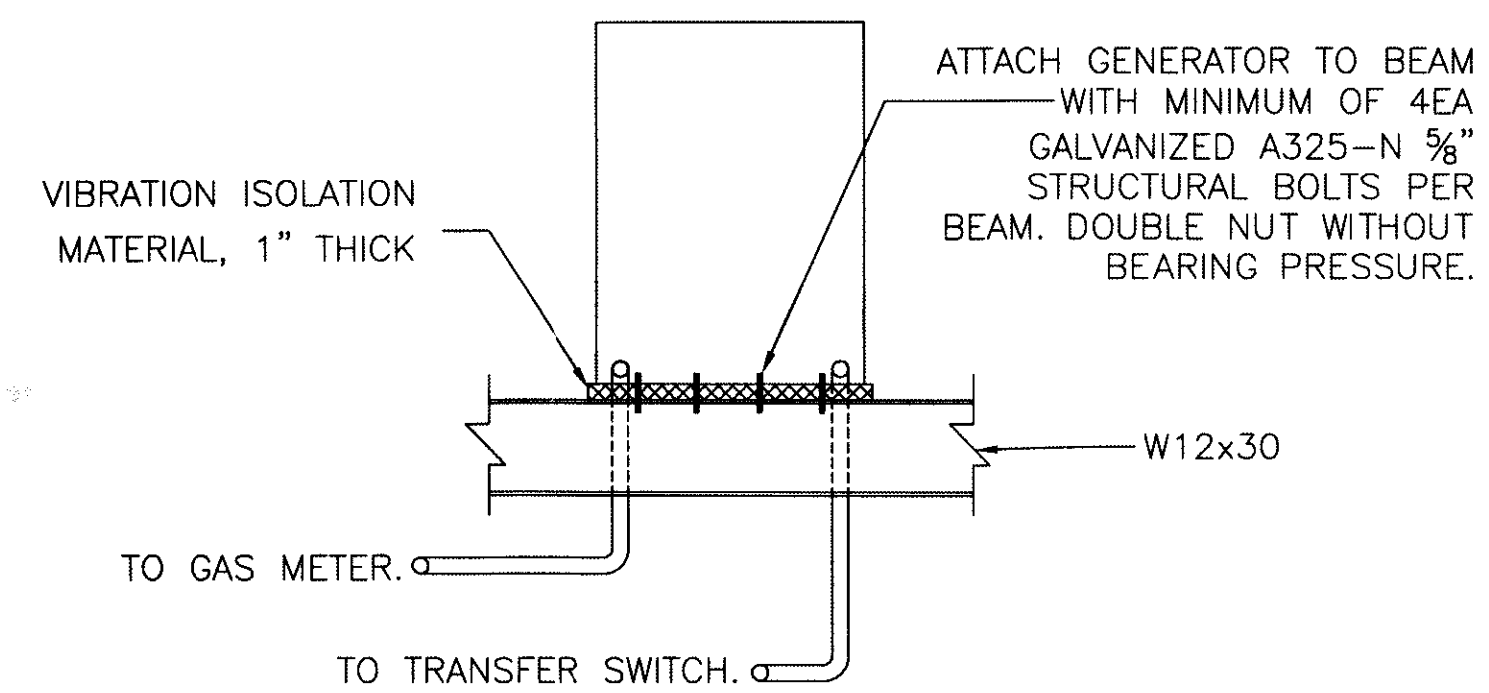
2 TYPICAL GENERATOR SETUP Scale: Not To Scale
