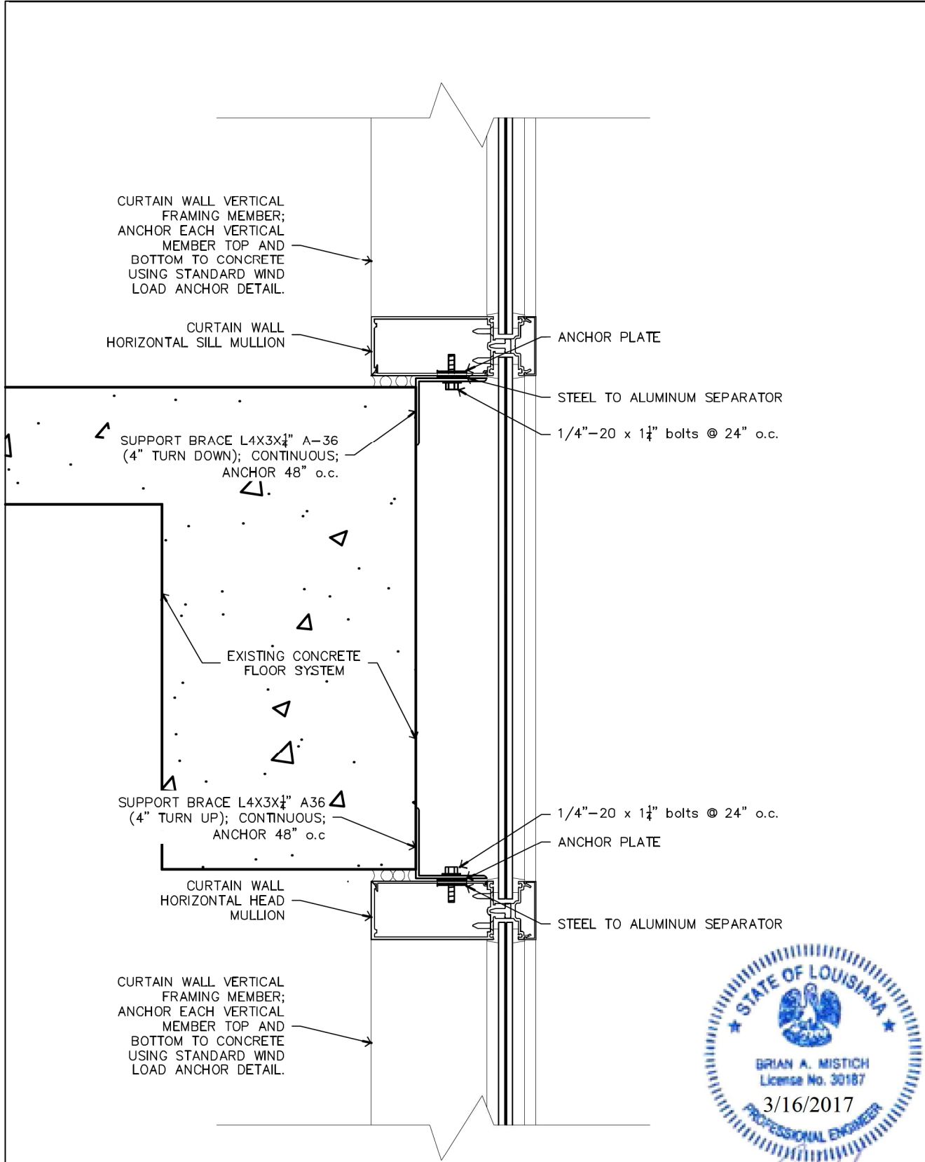
Detail—Curtainwall @ 2nd Floor
