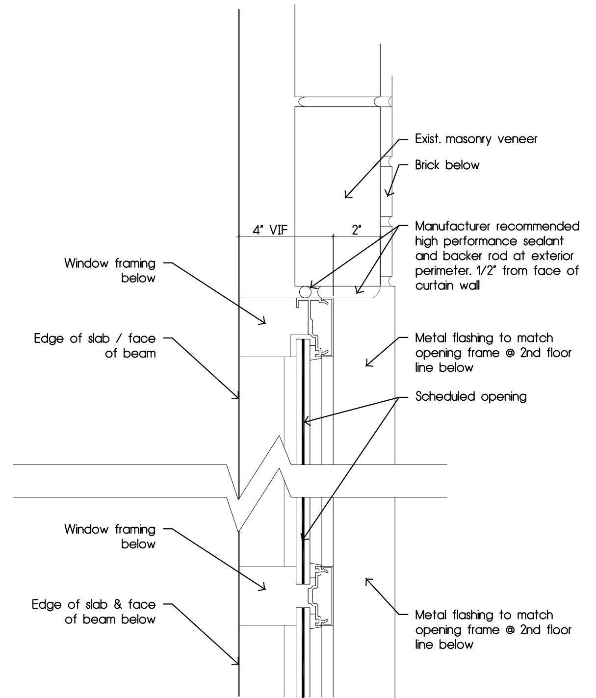
Jamb Detail-Curtainwall @ Structure
