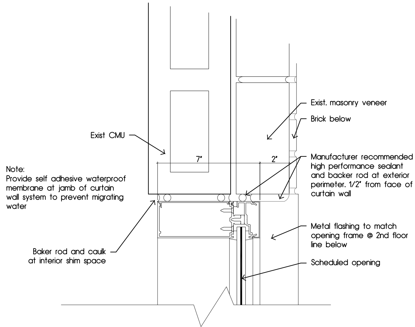
Jamb Detail-Curtainwall @ Occupied Space
