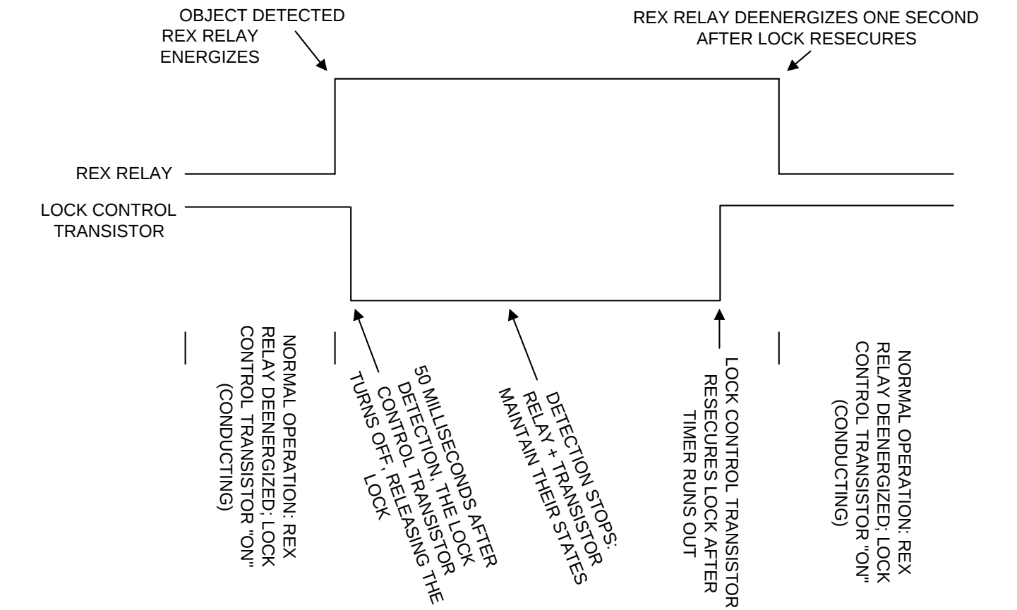
FIG. 8: OPERATIONAL TIMING CHART FOR XMS
