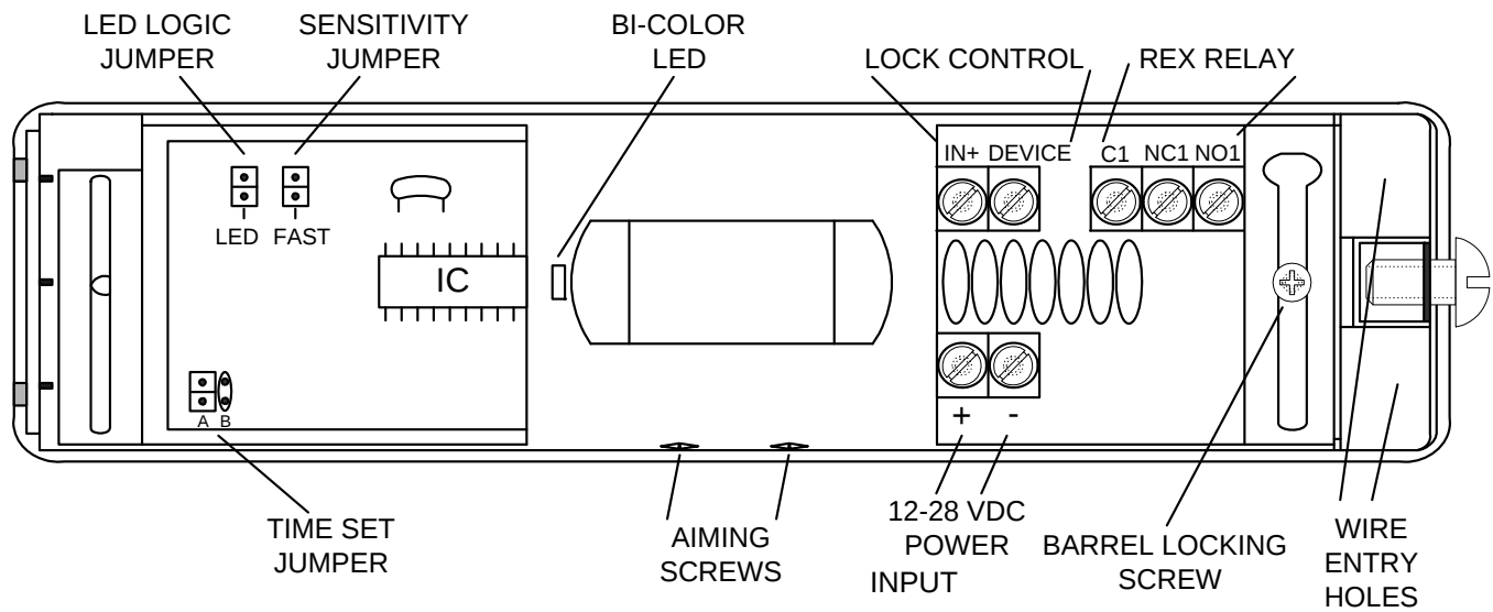
FIG. 2: XMS OVERVIEW
