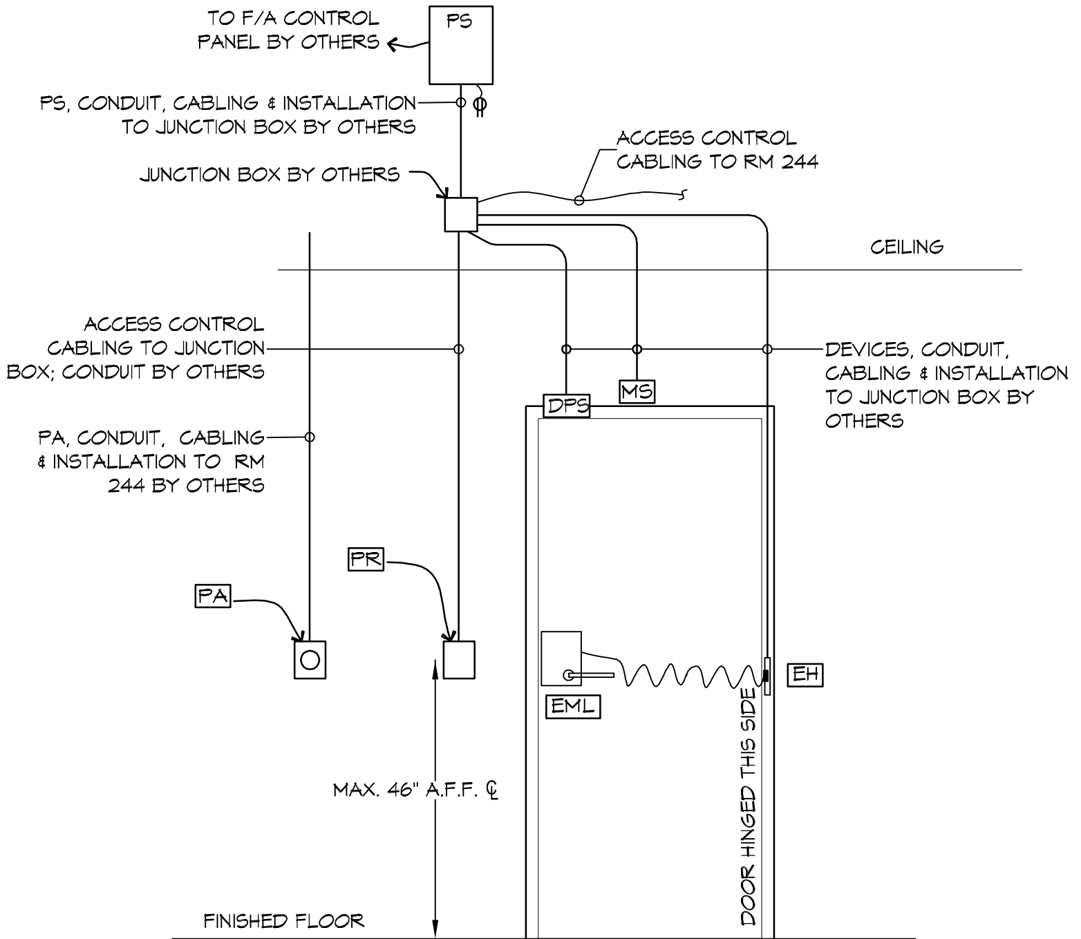
1 TYPICAL DOORS: 330
