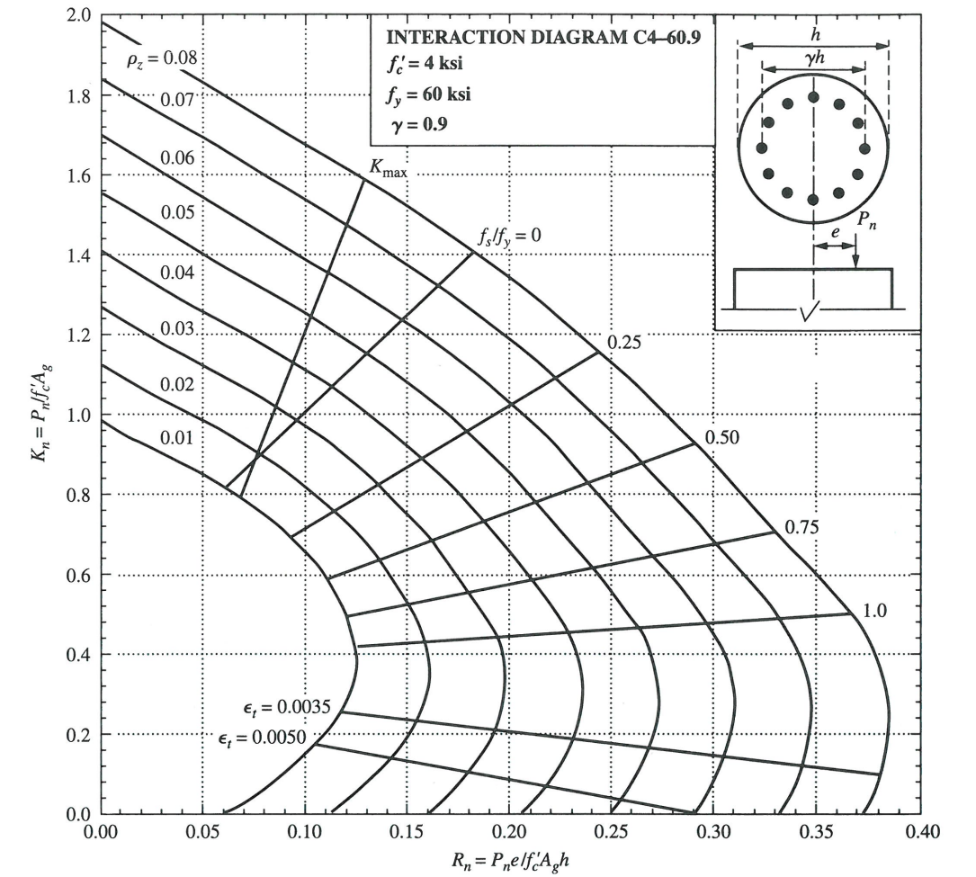
Graph 13 Column interaction diagrams for circular spiral columns.
