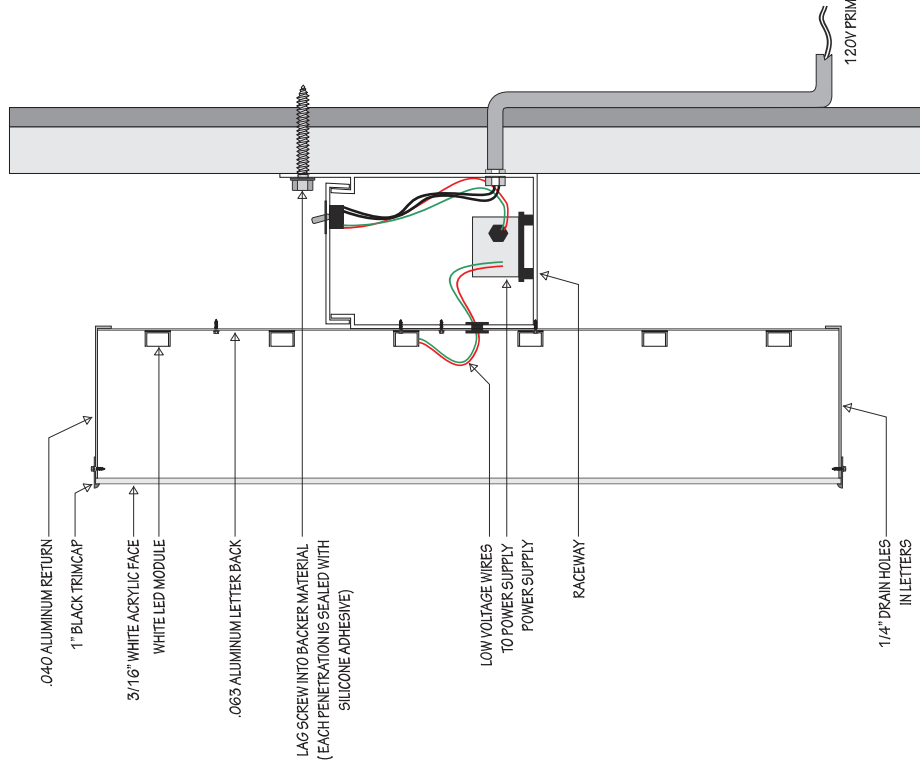
SECTION: S/F ILLUM. CHANNEL LETTERS
