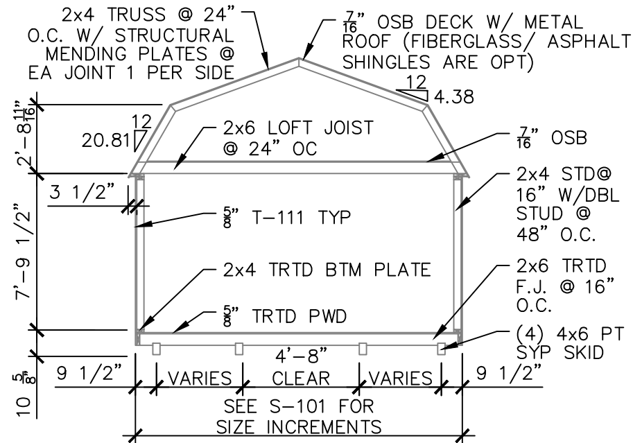
SECTION VIEW
