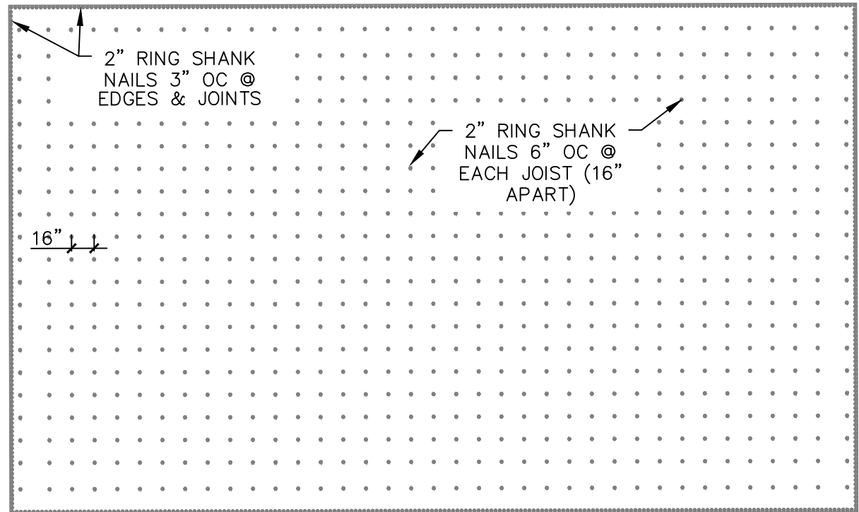
FLOOR SHEATHING PLAN
