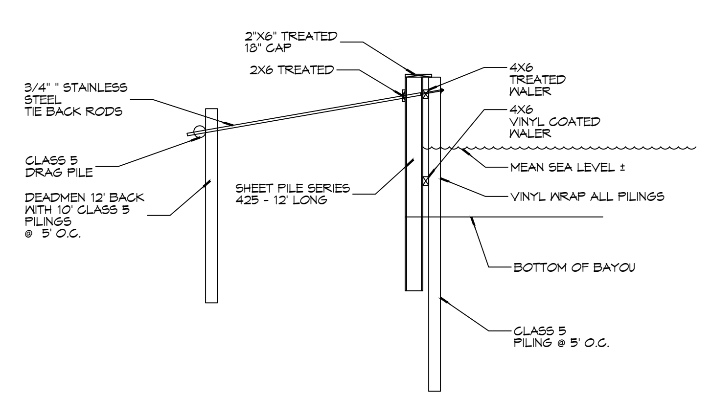
6 TYPICAL BULKHEAD SECTION SCALE: 3/16" = 1'-0"
